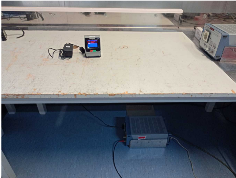
Photo 9: AC conducted emission test setup
