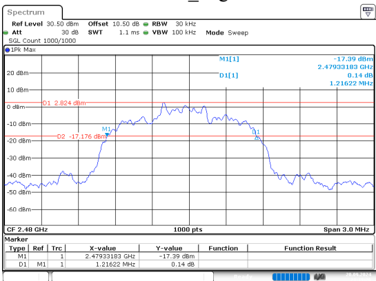
2DH1_High
