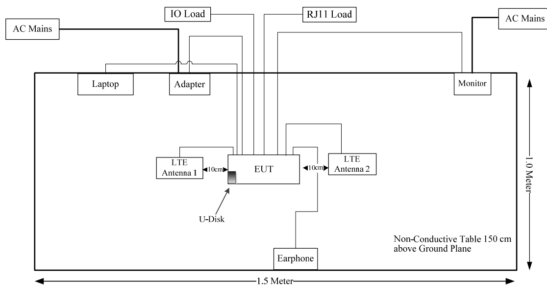
Configuration 2#:
