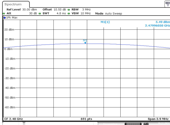
DH1_High
