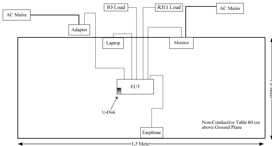
Configuration 3#:
