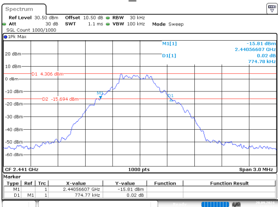
DH1_Middle
