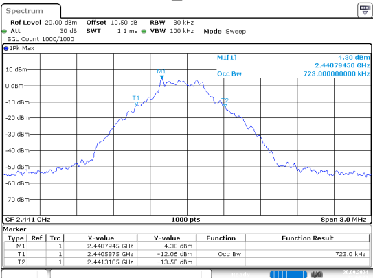
DH1_Middle
