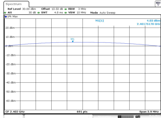
2DH1_Low
