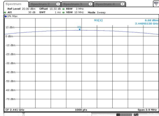
DH1_Middle
