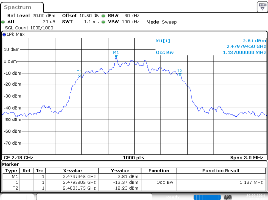
2DH1_High
