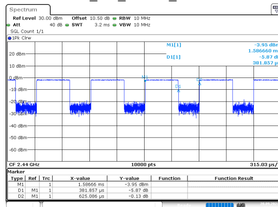
BLE_1M_Middle_Channel
