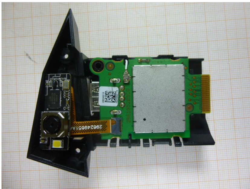
Photo 2: Cover removed
