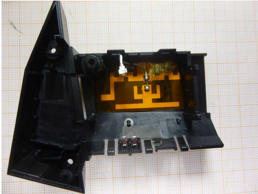
Photo 3: Antenna
