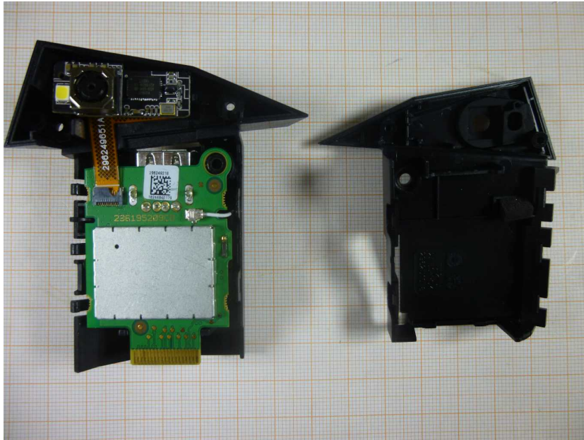
Photo 1: Cover removed
