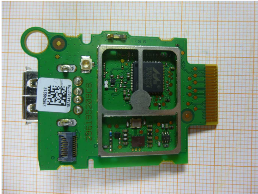
Photo 11: RF PCB front side view, shielding removed
