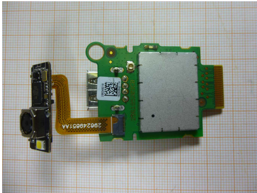
Photo 7: RF PCB front side view
