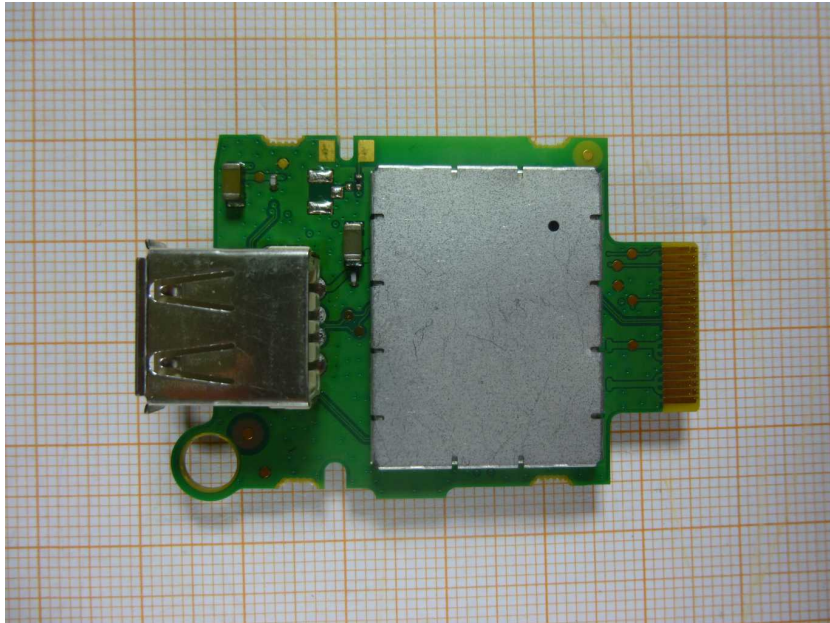
Photo 9: RF PCB back side view
