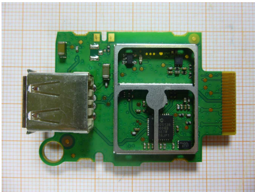
Photo 10: RF PCB back side view, shielding removed
