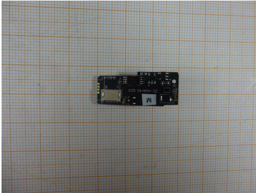
Photo 5: Camera PCB back side view
