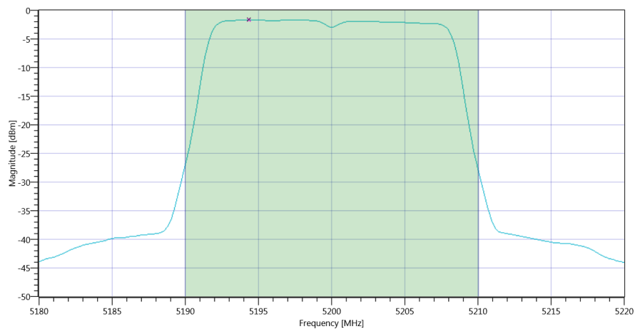
Plot_FCC Part 15.407 Max Output Power and PSD ~ WLAN5Gx a mode U-NII-1 Max OP and PSD_30082019_170144.png
