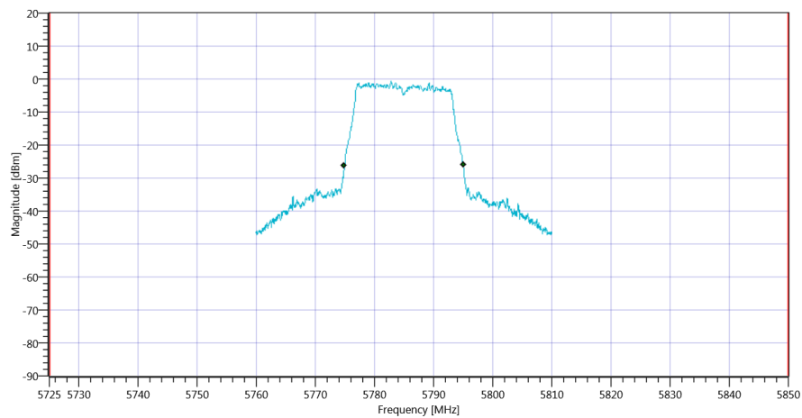
Plot_FCC Part 15.407 & ISSED Bandwidths ~ WLAN5Gx a mode U-NII-3_30082019_172054.png
