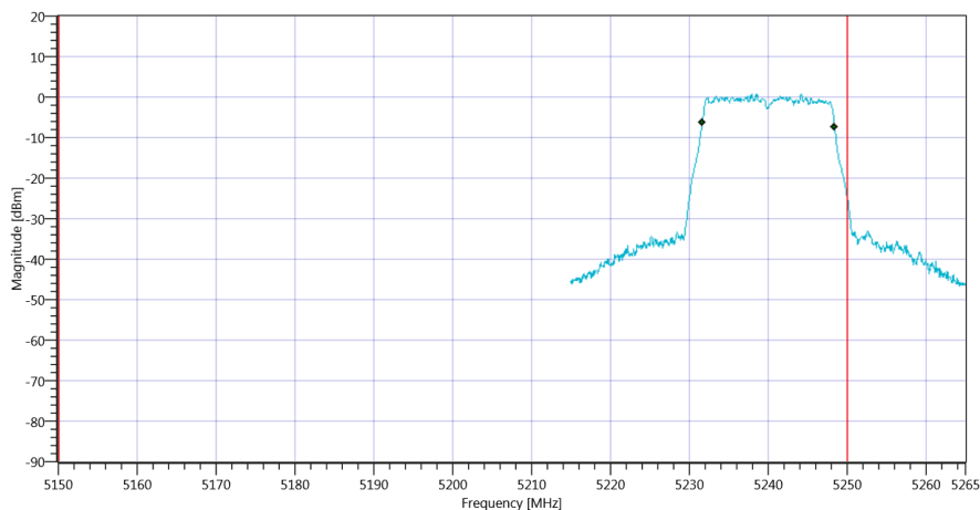
Plot_FCC Part 15.407 & ISCED Bandwidths ~ WLAN5Gx a mode U-NII-1_30082019_170457.png
