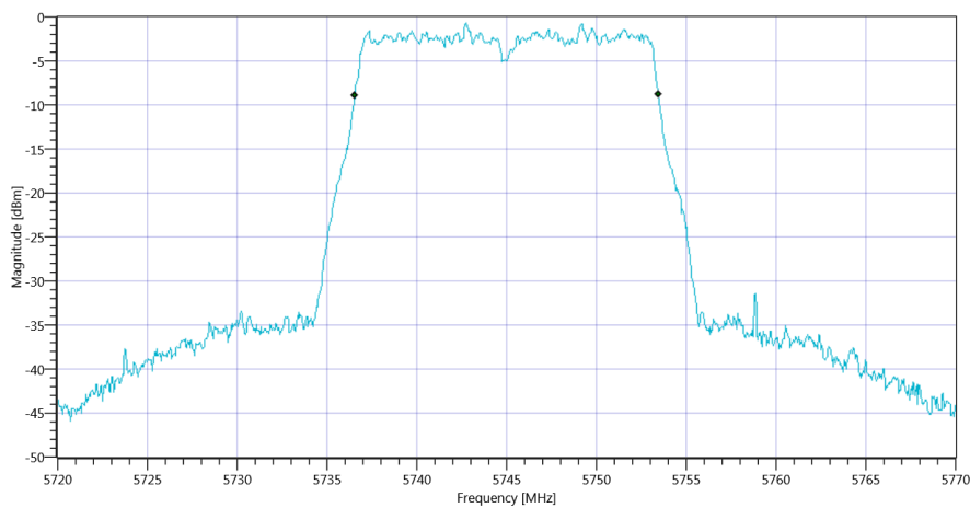
Plot_FCC Part 15.407 & ISCED Bandwidths ~ WLAN5Gx a mode U-NII-3 99PCT_30082019_171650.png
