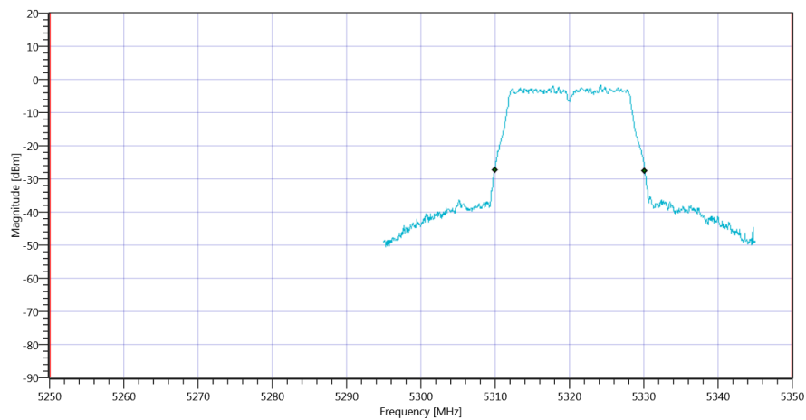
Plot_FCC Part 15.407 & ISSED Bandwidths ~ WLAN5Gx a mode U-NII-2A_30082019_171311.png
