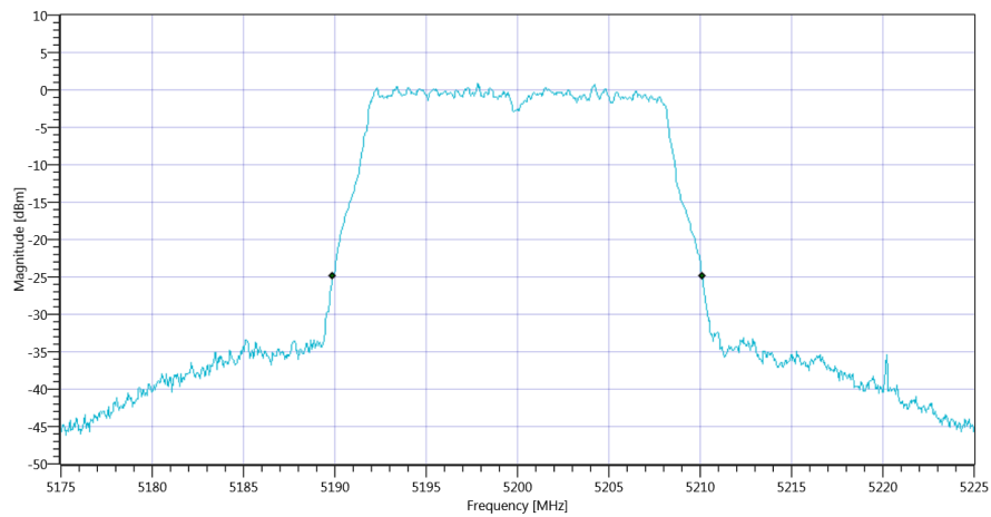
Plot_FCC Part 15.407 & ISM Bandwidths ~ WLAN5Gx a mode U-NII-1 26dB_30082019_170257.png
