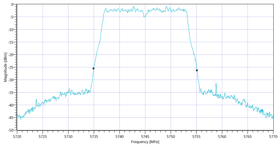
Plot_FCC Part 15.407 & ISSED Bandwidths ~ WLAN5Gx a mode U-NII-3 26dB_30082019_171656.png
