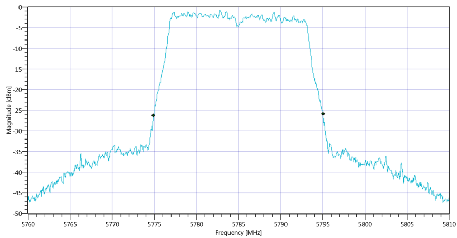
Plot_FCC Part 15.407 & ISSED Bandwidths ~ WLAN5Gx a mode U-NII-3 26dB_30082019_172051.png
