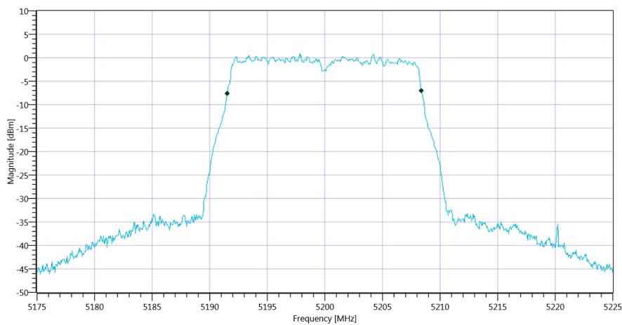
Plot_FCC Part 15.407 & ISCED Bandwidths ~ WLAN5Gx a mode U-NII-1 99PCT_30082019_170250.png
