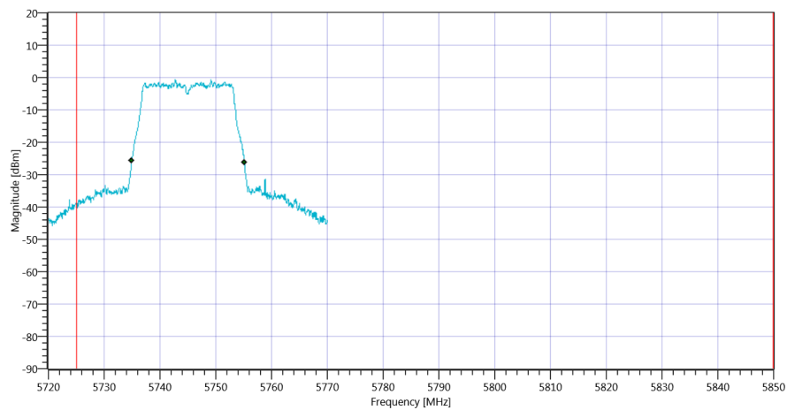
Plot_FCC Part 15.407 & ISSED Bandwidths ~ WLAN5Gx a mode U-NII-3_30082019_171659.png
