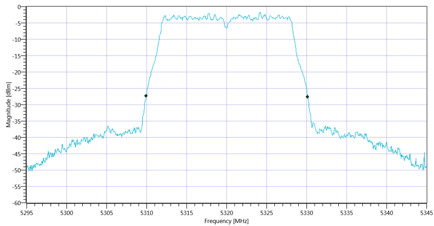
Plot_FCC Part 15.407 & ISSED Bandwidths ~ WLAN5Gx a mode U-NII-2A 26dB_30082019_171308.png
