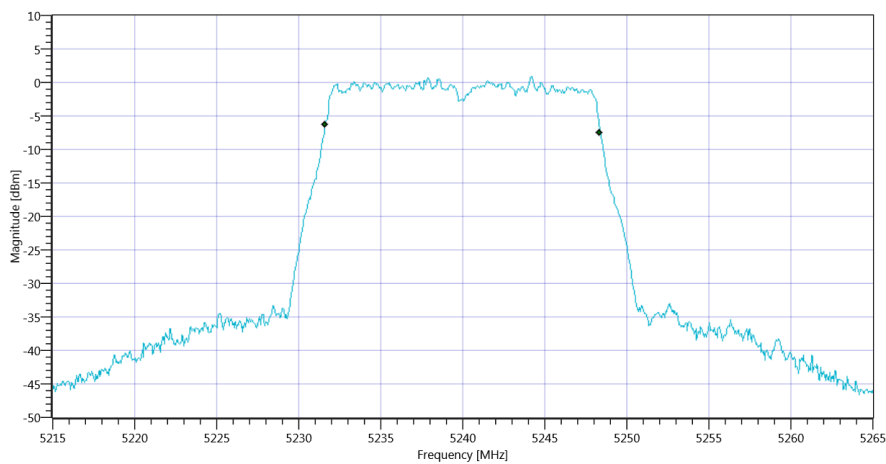
Plot_FCC Part 15.407 & ISCED Bandwidths ~ WLAN5Gx a mode U-NII-1 99PCT_30082019_170454.png
