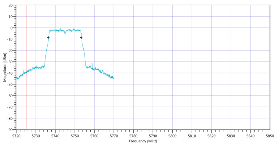
Plot_FCC Part 15.407 & ISCED Bandwidths ~ WLAN5Gx a mode U-NII-3_30082019_171653.png
