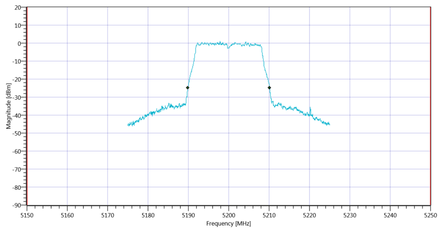
Plot_FCC Part 15.407 & ISM Bandwidths ~ WLAN5Gx a mode U-NII-1_30082019_170259.png
