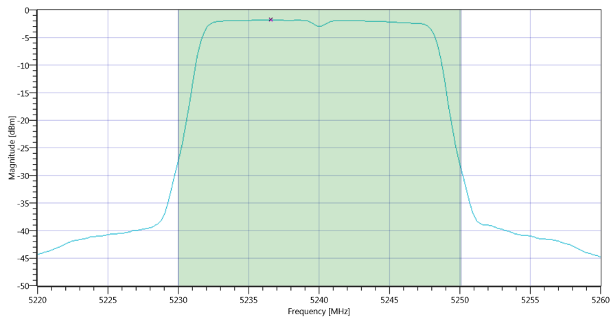
Plot_FCC Part 15.407 Max Output Power and PSD ~ WLAN5Gx a mode U-NII-1 Max OP and PSD_30082019_170353.png
