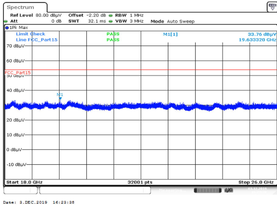
Plot 5: 18 GHz to 26 GHz; vertical & horizontal polarization; U-NII-2C; middle channel
