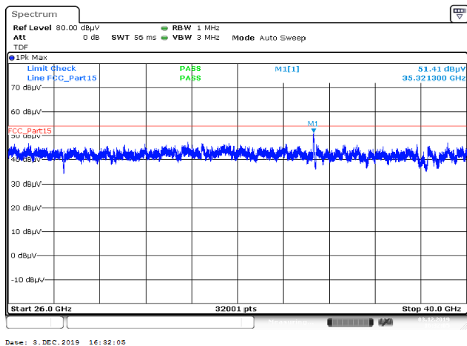
Plot 6: 26 GHz to 40 GHz; vertical & horizontal polarization; U-NII-2C; middle channel
