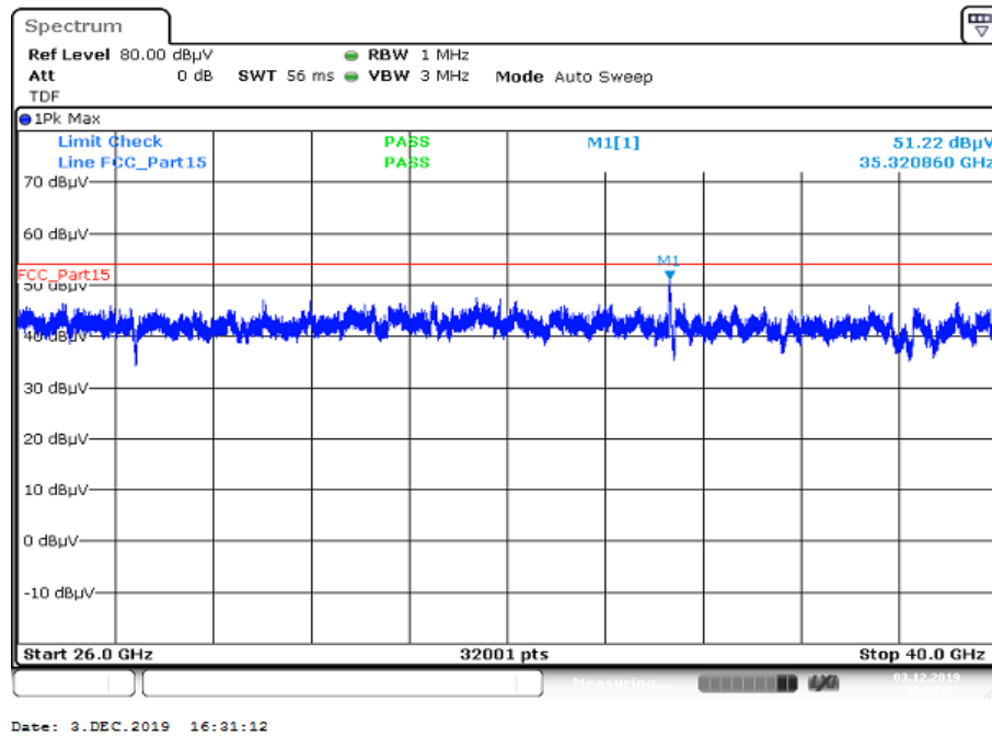
Plot 3: 26 GHz to 40 GHz; vertical & horizontal polarization; U-NII-2C; lowest channel
