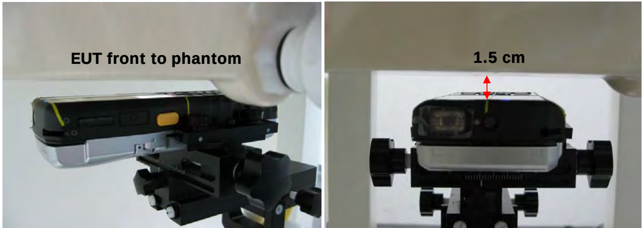
Fig.7 Body worn- EUT front to flat phantom and distance between flat phantom and mobile phone is 1.5 cm
