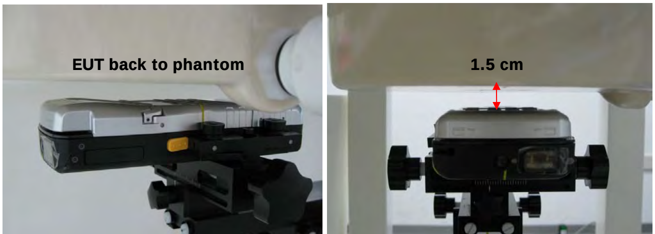
Fig.8 Body worn- EUT back to flat phantom and distance between flat phantom and mobile phone is 1.5 cm
