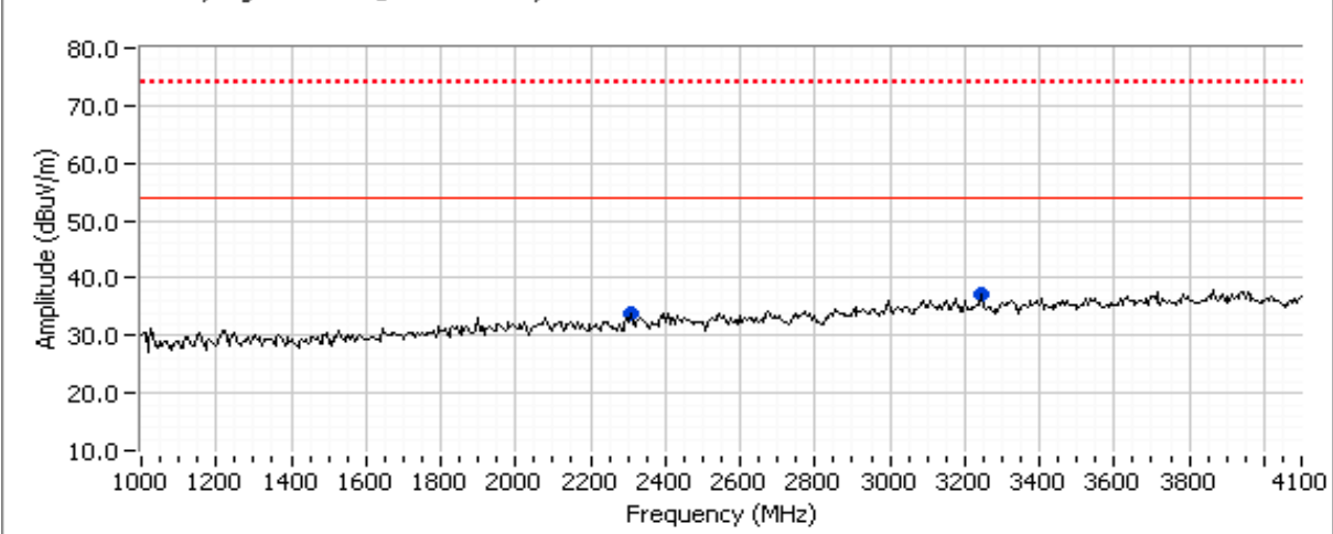
1000 - 4100 MHz, High Channel @ 404.55 MHz, EUT Flat Orientation
