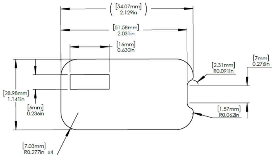
Figure 1: Dimensions of the Label and Transparent Window
