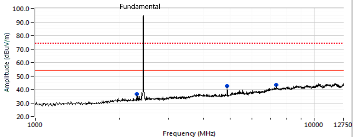
2440 MHz - Flat
