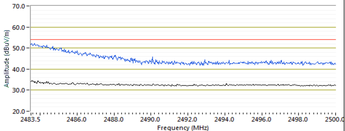
RB 1 MHz; VB 3 kHz (Blue); RB 1 MHz; VB 3 MHz (Black) Vert
