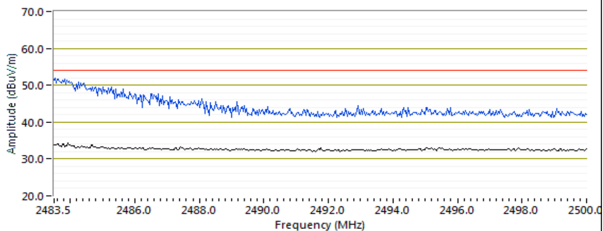
RB 1 MHz; VB 3 kHz (Blue); RB 1 MHz; VB 3 MHz (Black) Horiz
