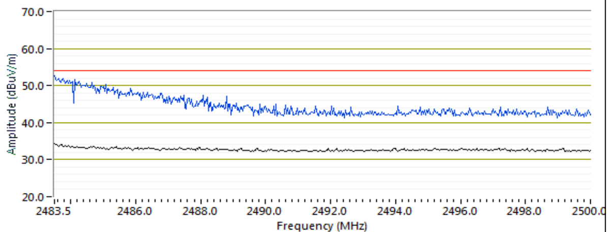
RB 1 MHz; VB 3 kHz (Blue); RB 1 MHz; VB 3 MHz (Black) Horiz (flat)
