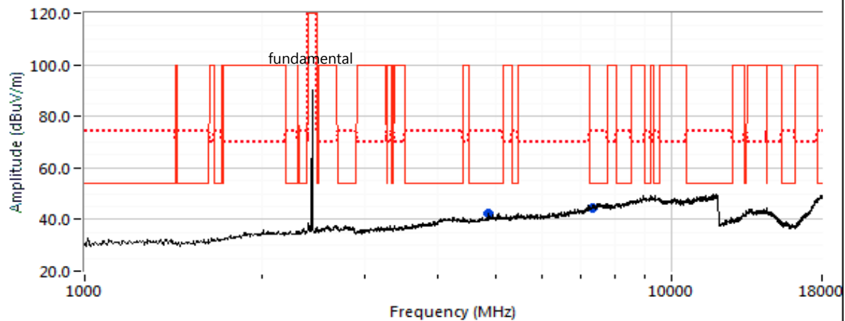
2440 MHz (side)
