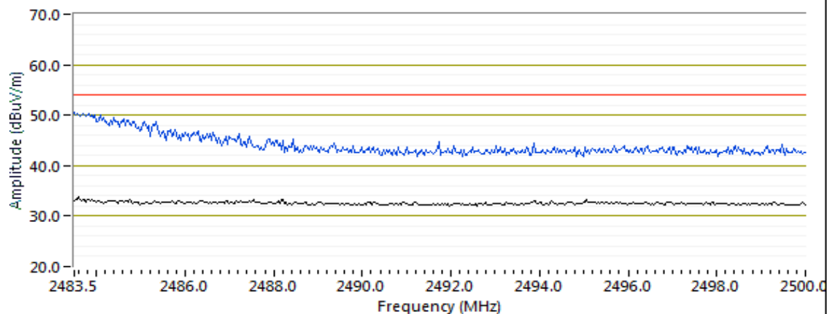
RB 1 MHz; VB 3 kHz (Blue); RB 1 MHz; VB 3 MHz (Black) Vert (side)
