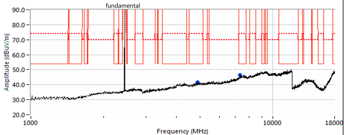
2440 MHz (flat)
