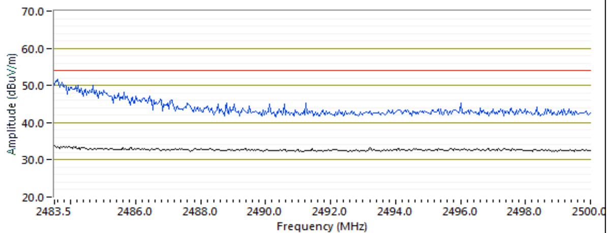
RB 1 MHz; VB 3 kHz (Blue); RB 1 MHz; VB 3 MHz (Black) Horiz (side)
