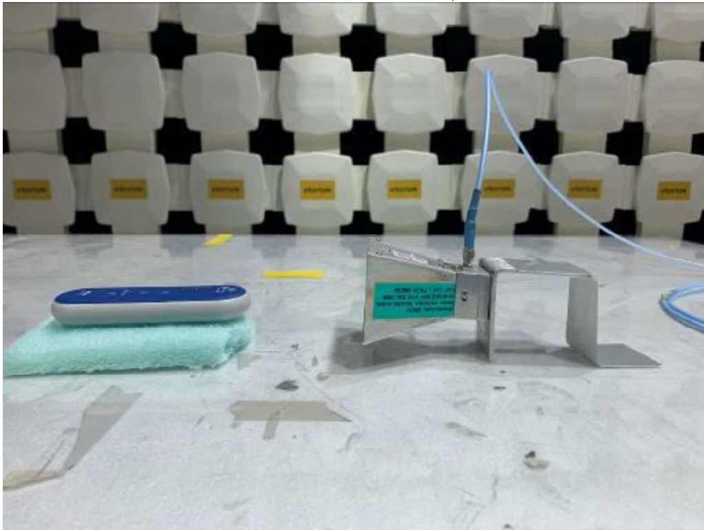
Manual scan at a distance of 10 cm, 13-25 GHz
