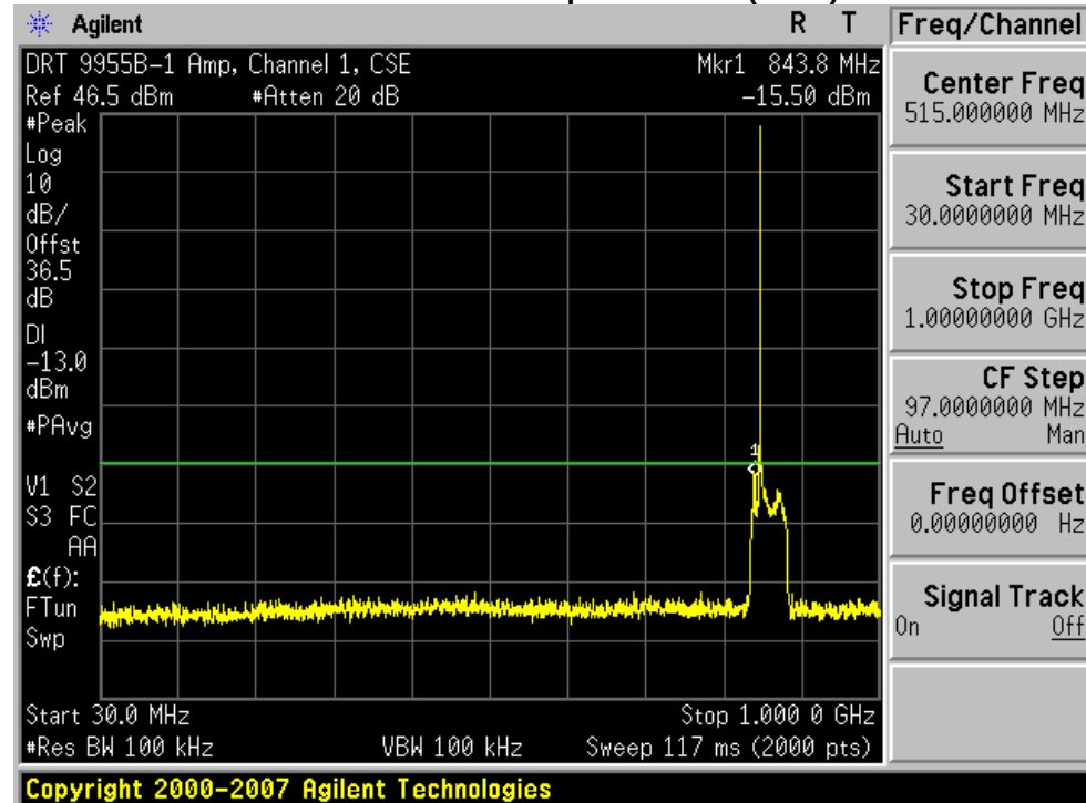
Plot 7-1. Conducted Spurious Plot (Ch. 1)
