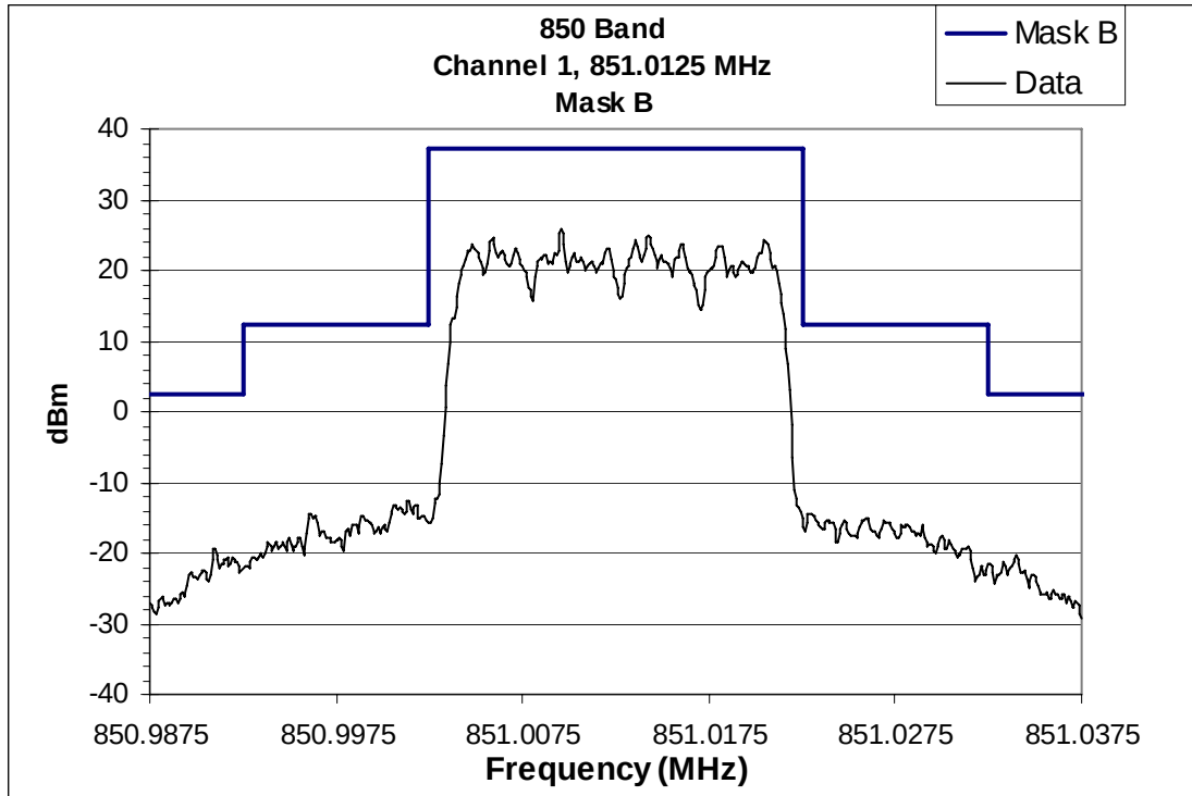
Figure 7-1: 850 Band Emission Mask, Channel 1 (S90.210(b))
