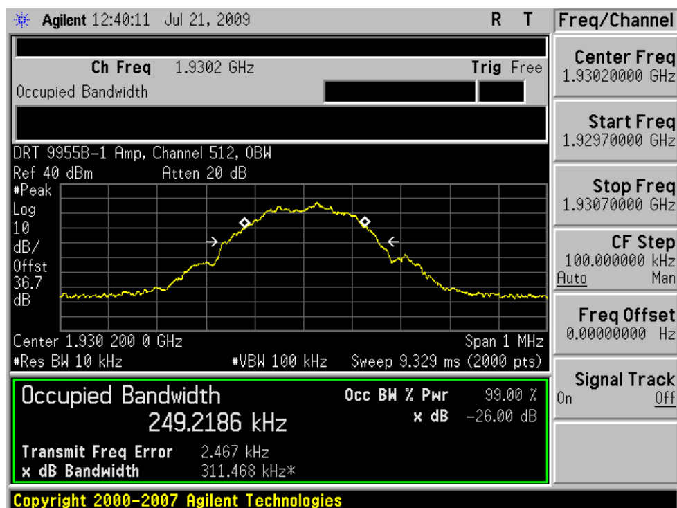
Plot 7-46. Occupied Bandwidth Plot (PCS GSM Mode – Ch. 512)
