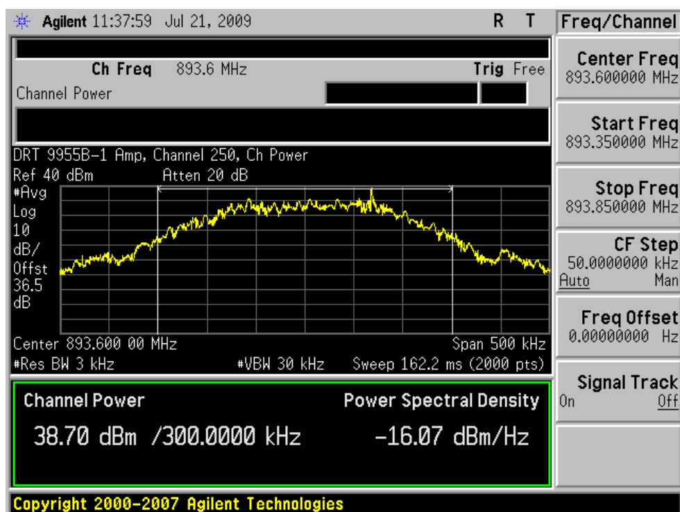
Plot 7-16. Channel Power (Cellular GSM Mode – Ch. 250)
