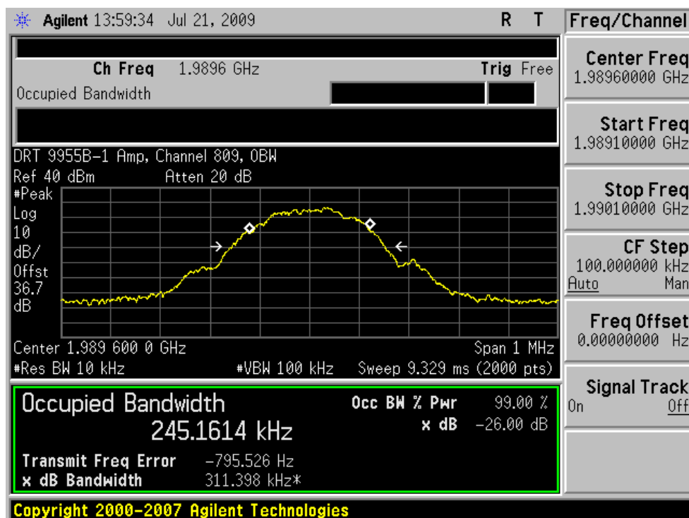
Plot 7-66. Occupied Bandwidth Plot (PCS GSM Mode – Ch. 809)
