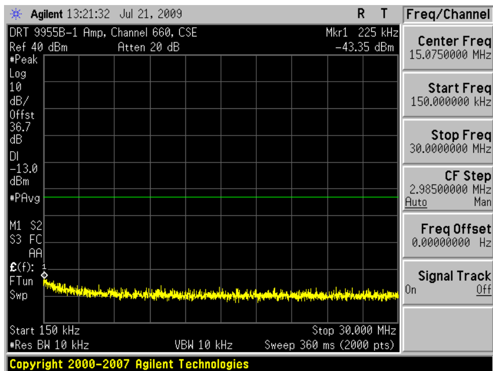
Plot 7-48. Conducted Spurious Plot (PCS GSM Mode – Ch. 660)
