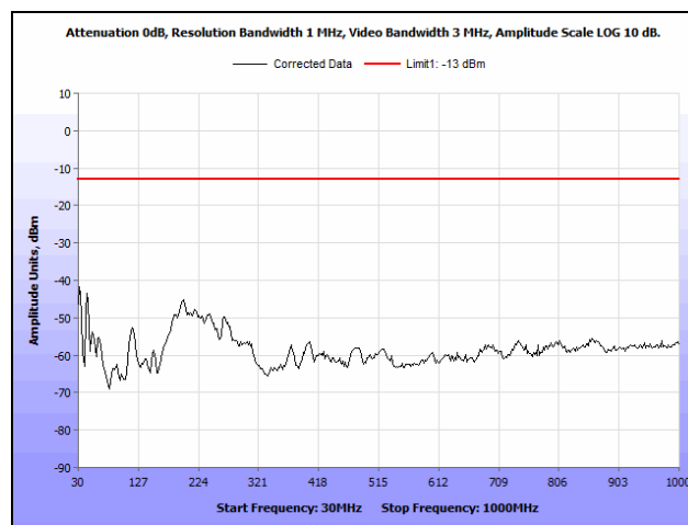
Plot 101. Radiated Spurious Emissions, High Channel, 30 MHz – 1 GHz, Part 24
