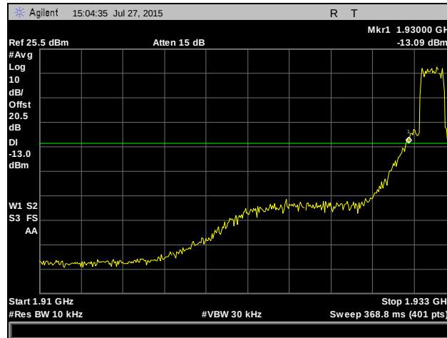
Plot 142. Conducted Band Edge, CDMA, Low Channel, Part 24
