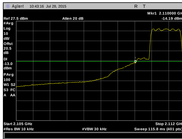
Plot 124. Conducted Band Edge, CDMA, Low Channel, Part 27
