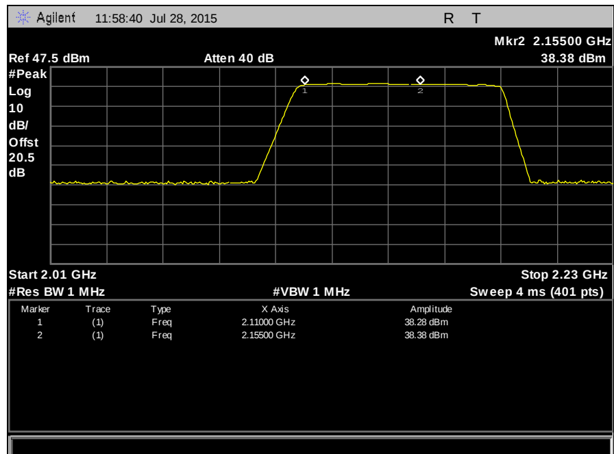
Plot 135. Filter Response with Marker Table, Part 27
