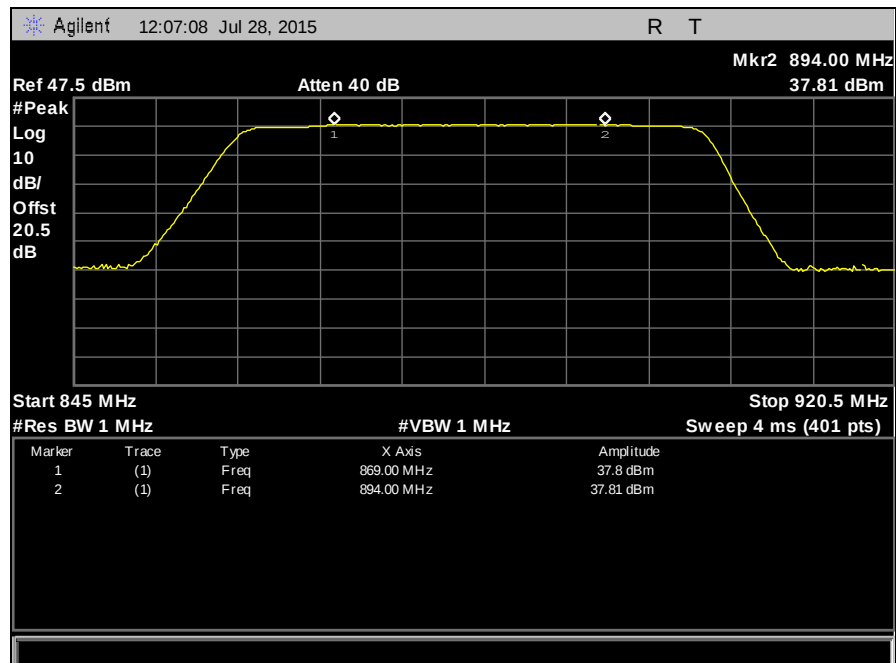
Plot 133. Filter Response with Marker Table, Part 22
