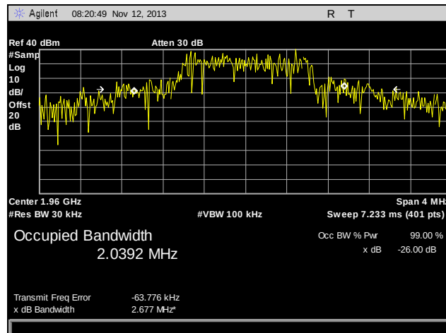
Plot 83. Occupied Bandwidth, CDMA, 1960 MHz, Output, Part 24
