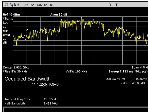
Plot 82. Occupied Bandwidth, CDMA, 1931.25 MHz, Output, Part 24
