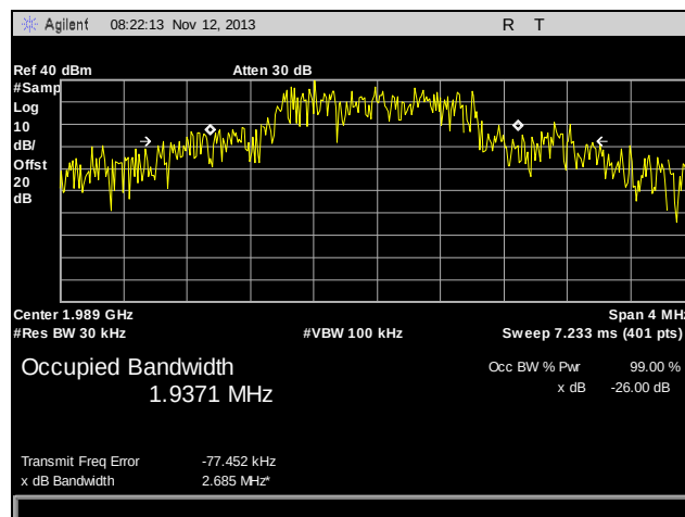
Plot 84. Occupied Bandwidth, CDMA, 1988.75 MHz, Output, Part 24
