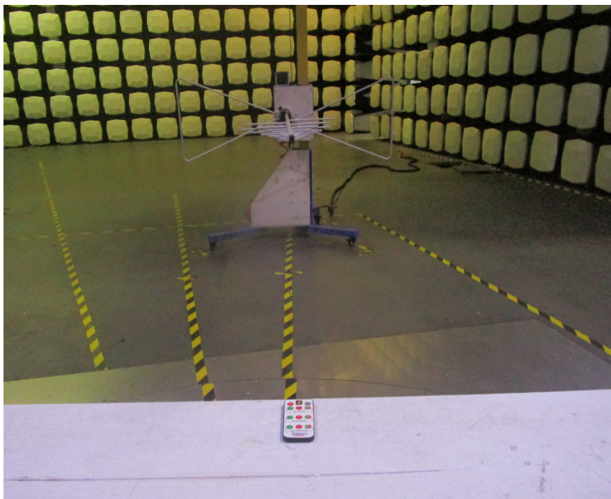
Radiated Emissions Below 1GHz
