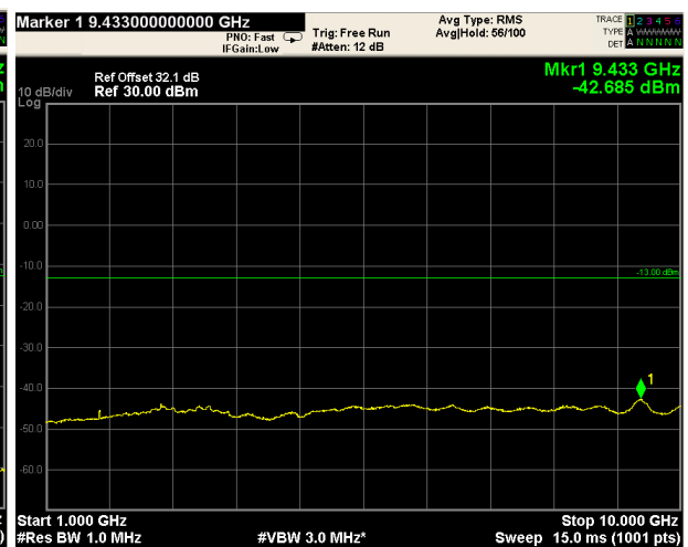
1GHz-10GHz
