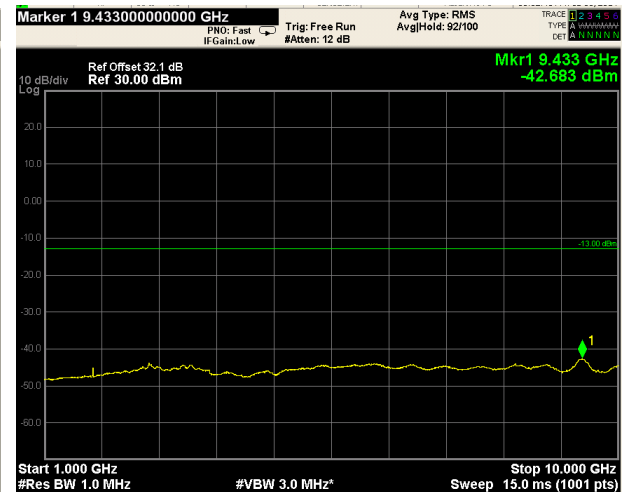
1GHz-10GHz
