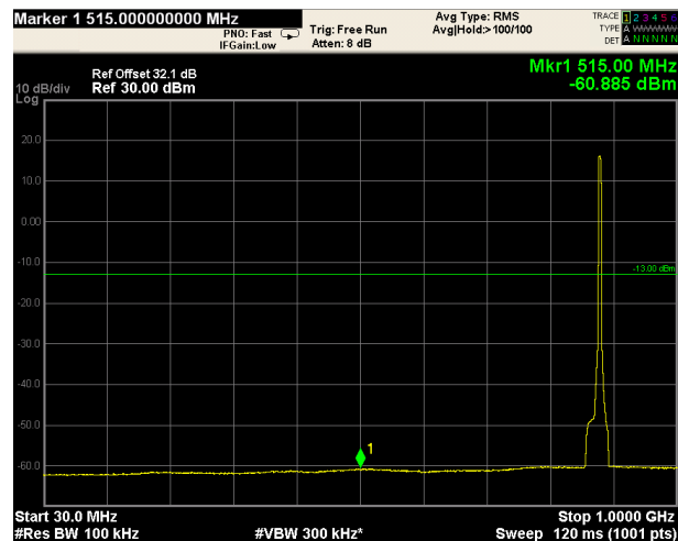
30MHz-1GHz
