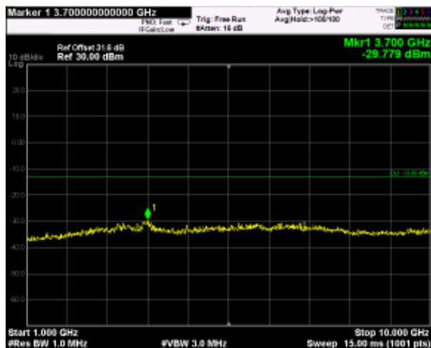
1GHz-10GHz
