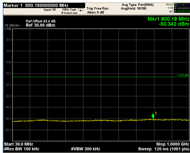
30MHz-1GHz
