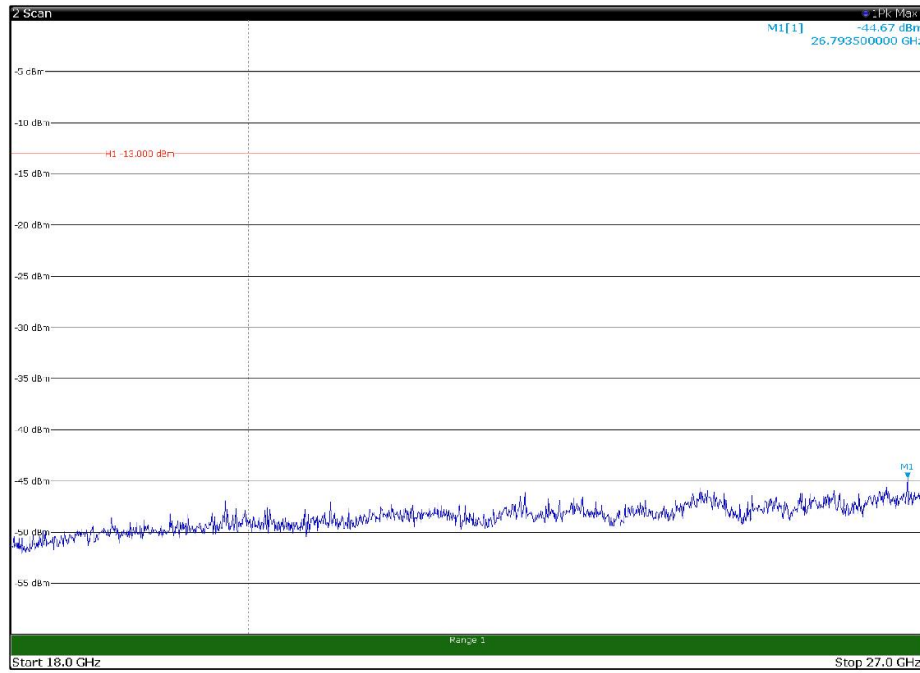
Channel: BOTTOM, Modulation: 256QAM, BW=5MHz, Range: 18GHz - 27GHz, Polarization: Horizontal
