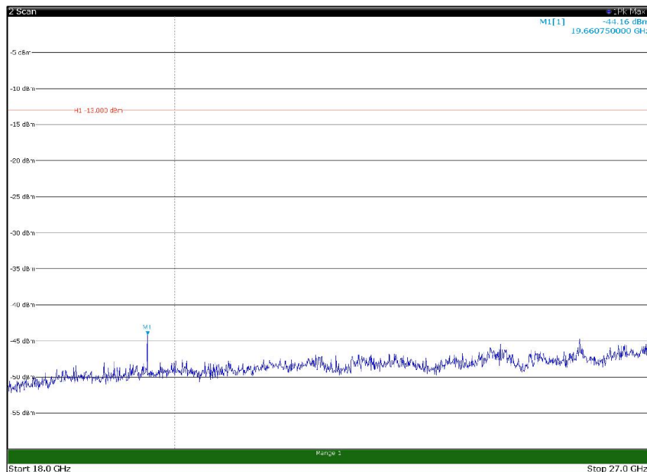
Channel: TOP, Modulation: 16QAM, BW=10MHz, Range: 18GHz - 27GHz, Polarization: Vertical
