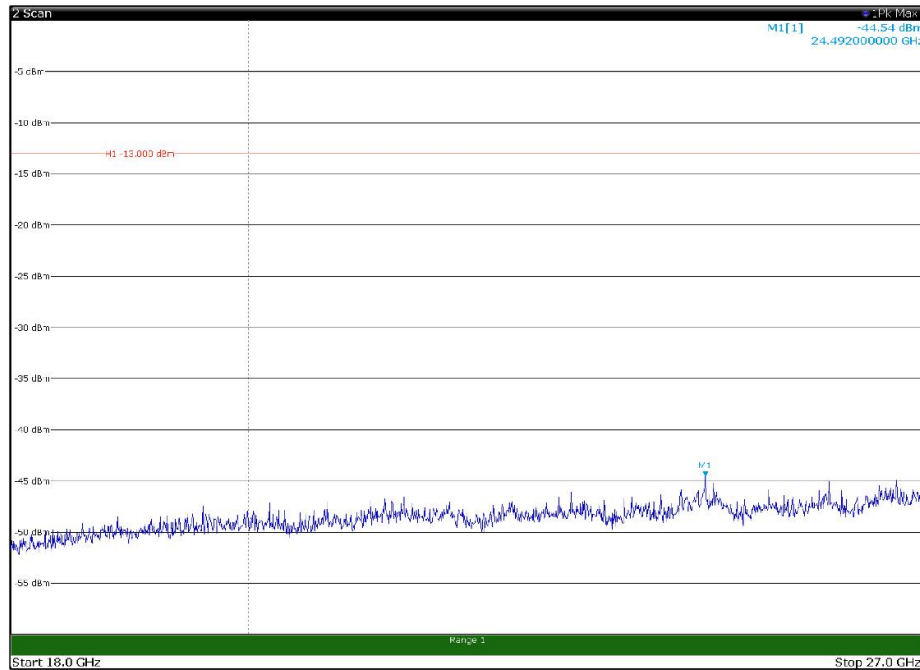
Channel: TOP, Modulation: 16QAM, BW=10MHz, Range: 18GHz - 27GHz, Polarization: Horizontal
