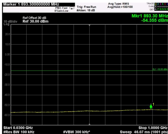
Channel: TOP, Modulation: QPSK, BW=10MHz, Range: Lower
