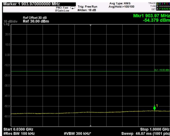
Channel: MIDDLE, Modulation: 64QAM, BW=10MHz, Range: Lower
