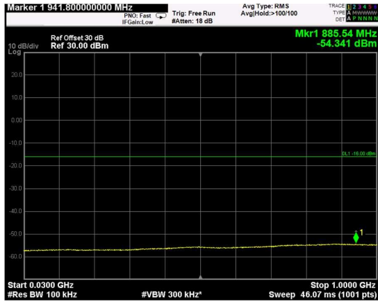
Channel: BOTTOM, Modulation: 64QAM, BW=15MHz, Range: Lower
