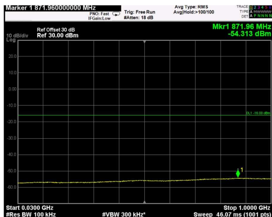
Channel: TOP, Modulation: 64QAM, BW=20MHz, Range: Lower
