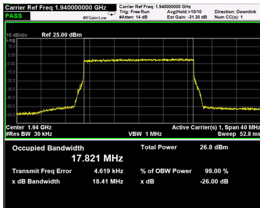
Channel: BOTTOM, Modulation: 64QAM, BW=20MHz
