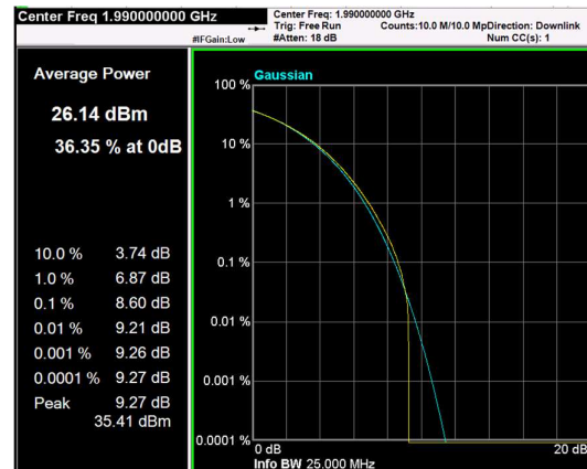
Channel: TOP, Modulation: QPSK, BW=10MHz, CCDF
