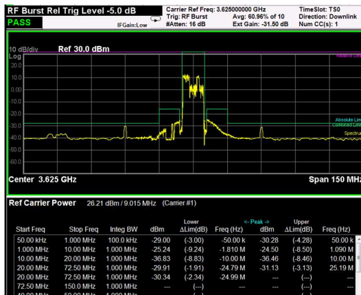
Middle Band Edge, 1 Carrier, Modulation: 256QAM, BW=10MHz
