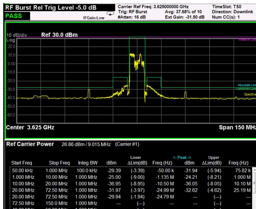
Middle Band Edge, 1 Carrier, Modulation: 16QAM, BW=10MHz
