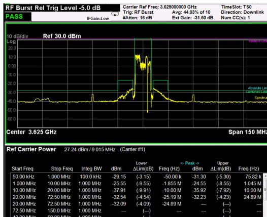
Middle Band Edge, 1 Carrier, Modulation: 64QAM, BW=10MHz
