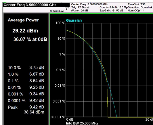
Channel: BOTTOM, Modulation: 64QAM, BW=20MHz, CCDF
