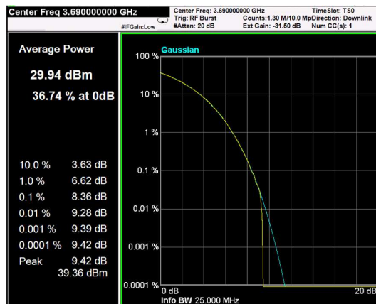
Channel: TOP, Modulation: QPSK, BW=20MHz, CCDF
