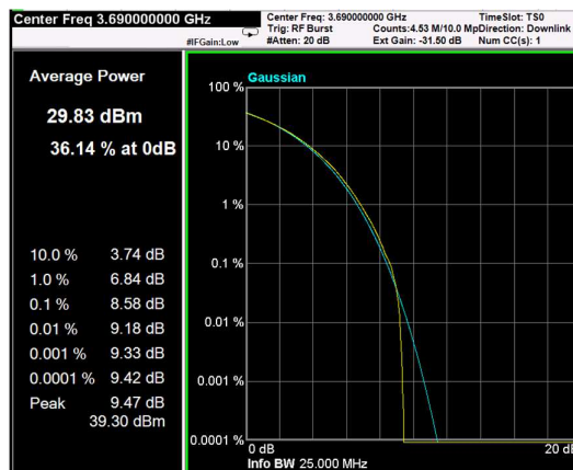
Channel: TOP, Modulation: 64QAM, BW=20MHz, CCDF
