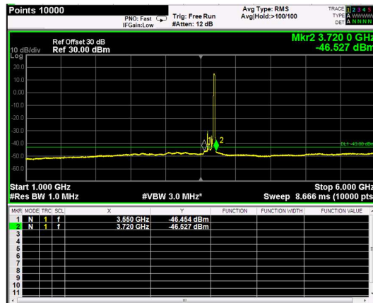
Channel: TOP, Modulation: 64QAM, BW=20MHz, Range: 1GHz - 6GHz
