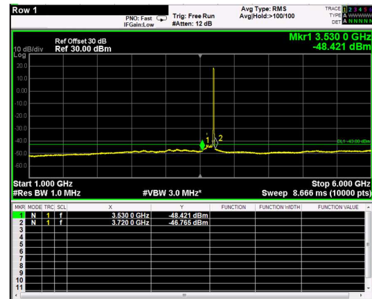
Channel: TOP, Modulation: 16QAM, BW=10MHz, Range: 1GHz - 6GHz
