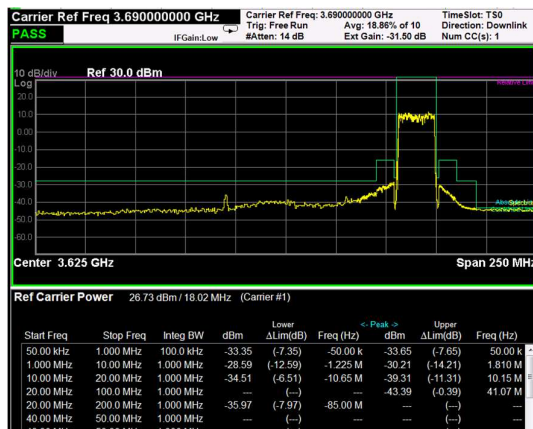
High Band Edge, 1 Carrier, Modulation: QPSK, BW=20MHz
