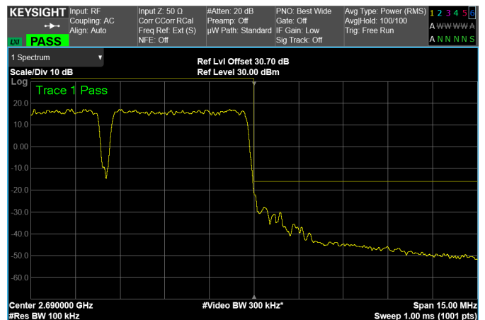
High Band Edge, 2 Carriers, Modulation: 64QAM, BW=5MHz
