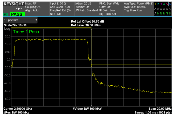
High Band Edge, 1 Carrier, Modulation: 64QAM, BW=10MHz
