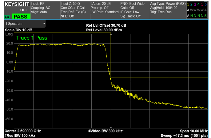
High Band Edge, 1 Carrier, Modulation: 64QAM, BW=5MHz
