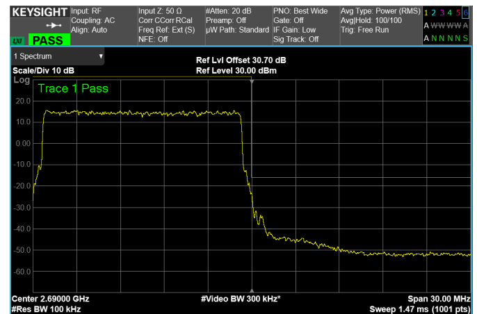
High Band Edge, 1 Carrier, Modulation: 64QAM, BW=15MHz
