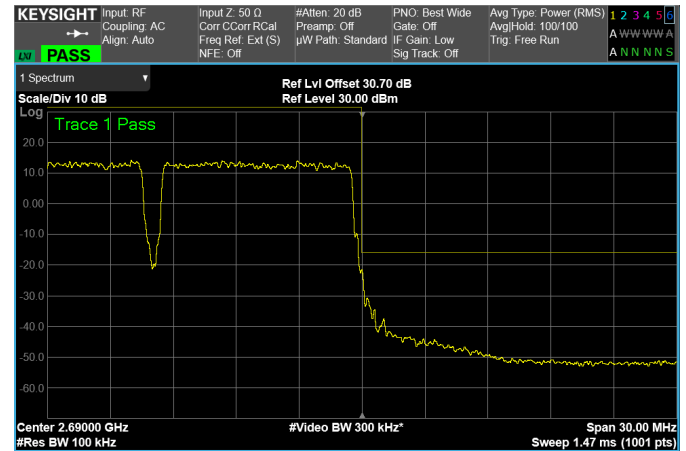
High Band Edge, 2 Carriers, Modulation: 64QAM, BW=10MHz
