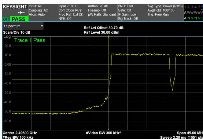
Low Band Edge, 2 Carriers, Modulation: 64QAM, BW=15MHz
