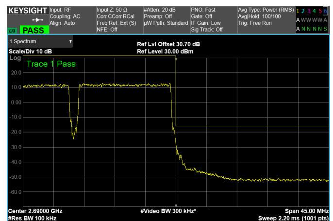
High Band Edge, 2 Carriers, Modulation: 64QAM, BW=15MHz
