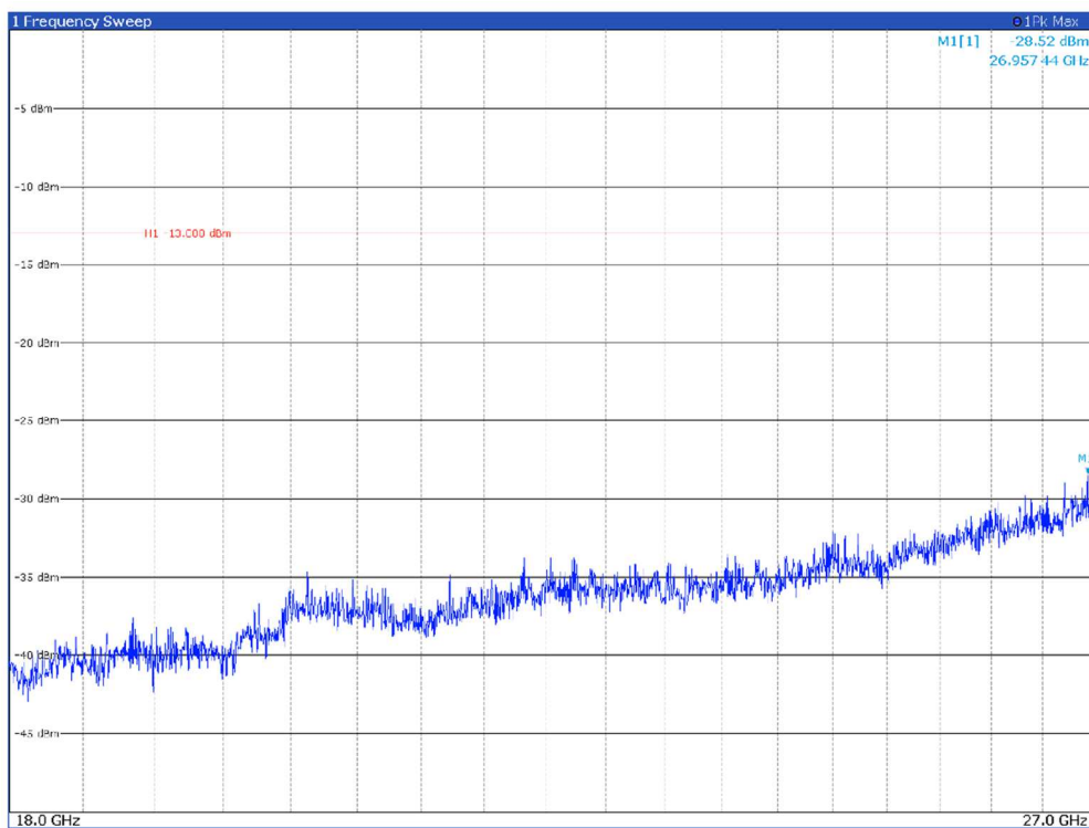
Channel: BOTTOM, Modulation: 64QAM, BW=15MHz, Range: 18GHz - 27GHz, Polarization: Vertical
