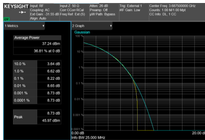
Channel: TOP, Modulation: 64QAM, BW=25MHz, CCDF
