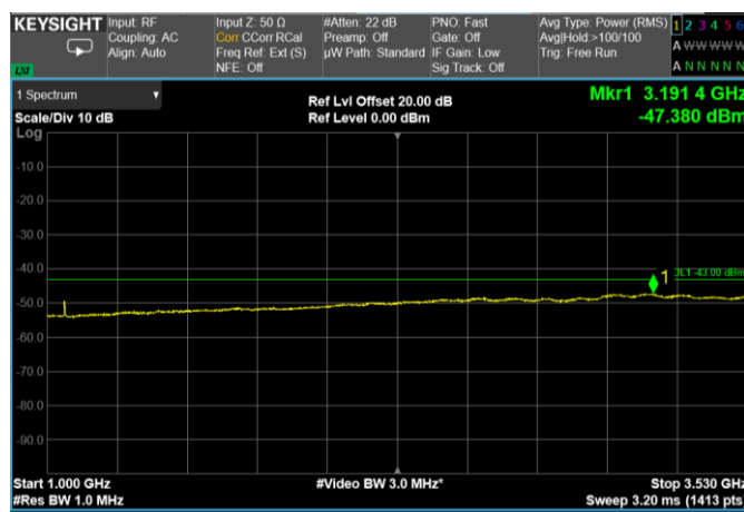
Channel: MIDDLE, Modulation: 64QAM, BW=5MHz, Range: 1000 MHz - 3530 MHz
