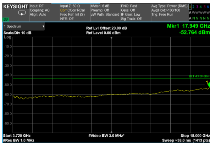
Channel: MIDDLE, Modulation: 64QAM, BW=5MHz, Range: 3720 MHz - 18 GHz
