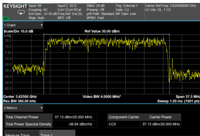
Channel: MIDDLE, Modulation: 64QAM, BW=25MHz, Channel Power
