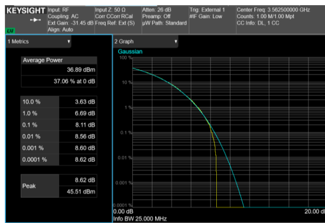
Channel: BOTTOM, Modulation: 64QAM, BW=25MHz, CCDF
