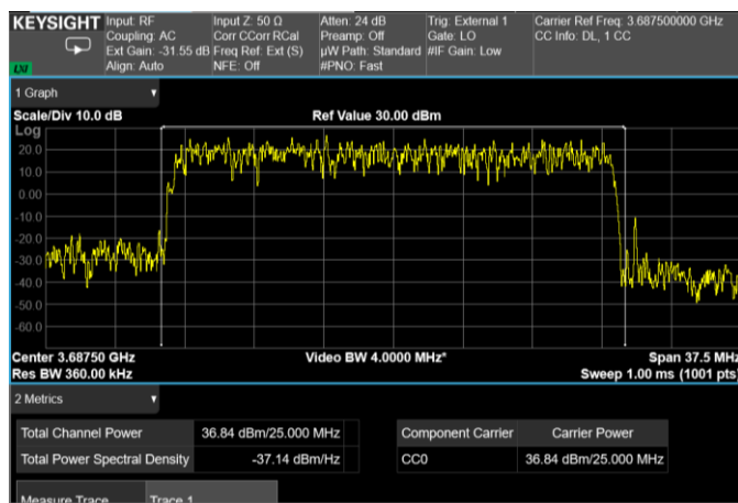
Channel: TOP, Modulation: 64QAM, BW=25MHz, Channel Power
