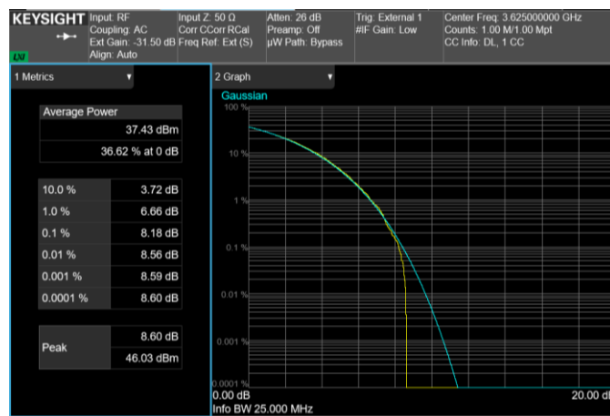
Channel: MIDDLE, Modulation: 64QAM, BW=25MHz, CCDF
