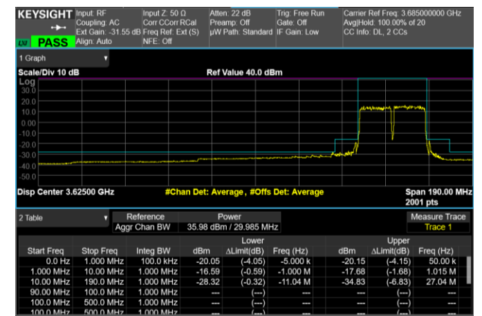
High Band Edge, 2 Carrier, Modulation: 64QAM, BW=15MHz
