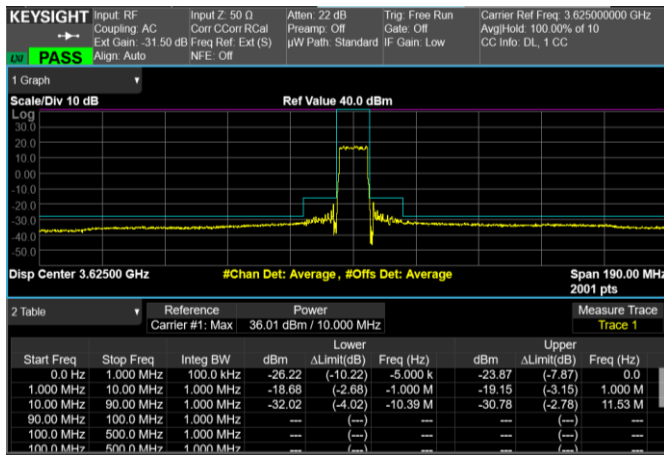
Middle Band Edge, 1 Carrier, Modulation: 64QAM, BW=10MHz
