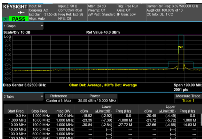
High Band Edge, 1 Carrier, Modulation: 64QAM, BW=5MHz
