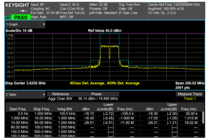
Middle Band Edge, 2 Carrier, Modulation: 64QAM, BW=10MHz
