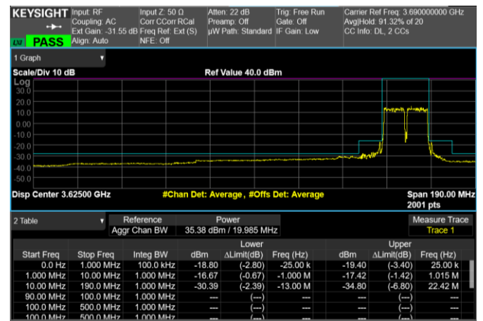
High Band Edge, 2 Carrier, Modulation: 64QAM, BW=10MHz
