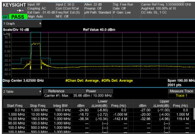
Low Band Edge, 1 Carrier, Modulation: 64QAM, BW=10MHz
