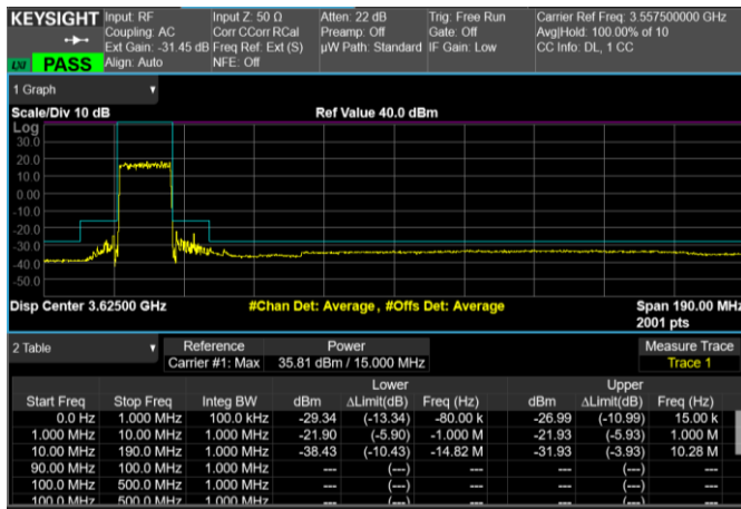
Low Band Edge, 1 Carrier, Modulation: 64QAM, BW=15MHz
