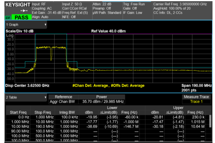
Low Band Edge, 2 Carrier, Modulation: 64QAM, BW=15MHz
