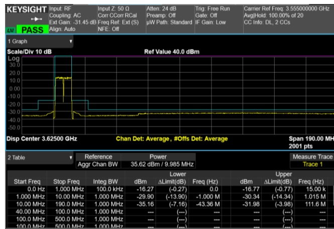
Low Band Edge, 2 Carrier, Modulation: 64QAM, BW=5MHz
