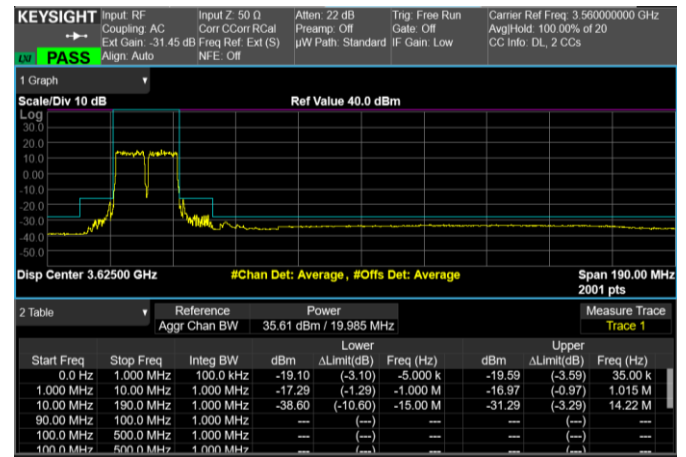
Low Band Edge, 2 Carrier, Modulation: 64QAM, BW=10MHz
