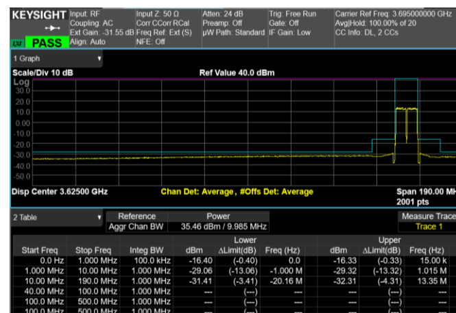
High Band Edge, 2 Carrier, Modulation: 64QAM, BW=5MHz
