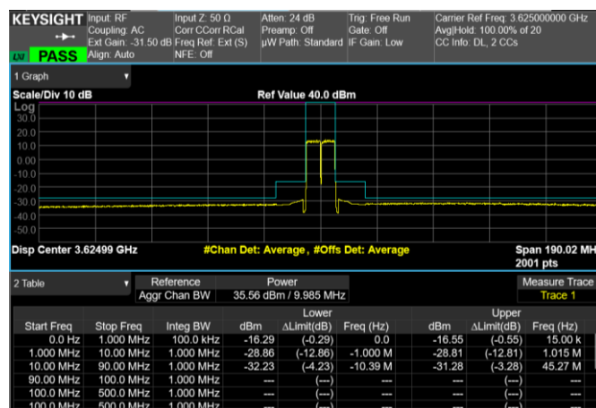
Middle Band Edge, 2 Carrier, Modulation: 64QAM, BW=5MHz
