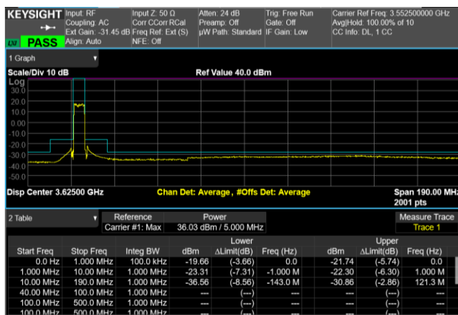
Low Band Edge, 1 Carrier, Modulation: 64QAM, BW=5MHz
