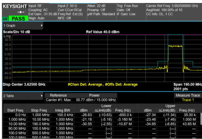
High Band Edge, 1 Carrier, Modulation: 64QAM, BW=15MHz
