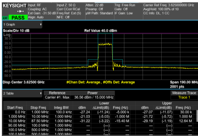
Middle Band Edge, 1 Carrier, Modulation: 64QAM, BW=15MHz
