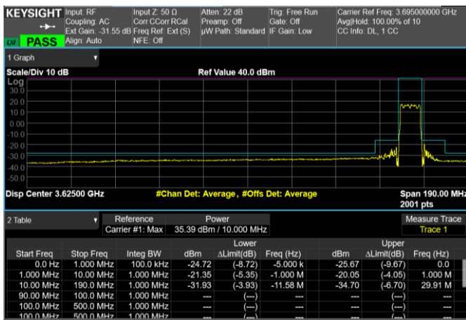
High Band Edge, 1 Carrier, Modulation: 64QAM, BW=10MHz
