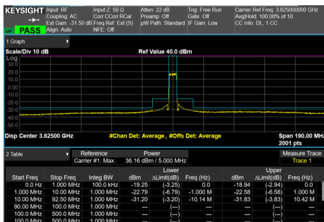
Middle Band Edge, 1 Carrier, Modulation: 64QAM, BW=5MHz
