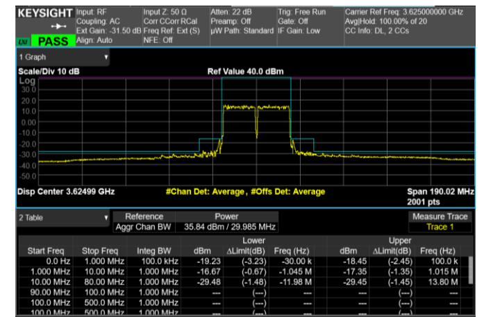
Middle Band Edge, 2 Carrier, Modulation: 64QAM, BW=15MHz
