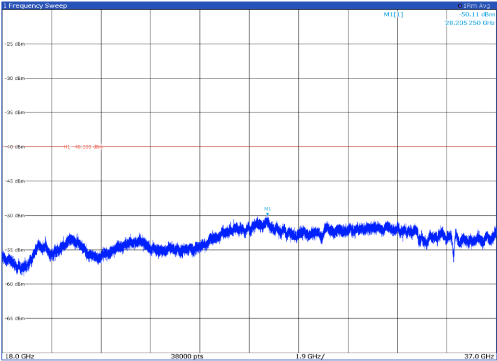
Channel: TOP, Modulation: 64QAM, BW=30 MHz, Range: 18 GHz-37 GHz, Polarization: Horizontal
