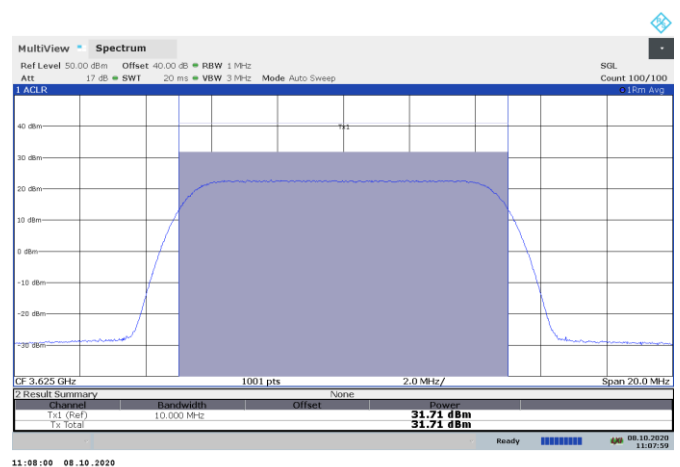
Figure 7.55-4: Output power and power density validation when maxEirp setting P_i = 32
