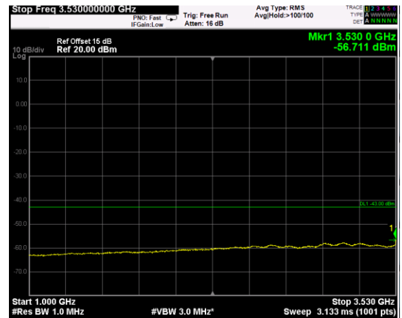
Channel: MIDDLE, Modulation: 16QAM, BW=10 MHz, Range: 1GHz - 3530MHz
