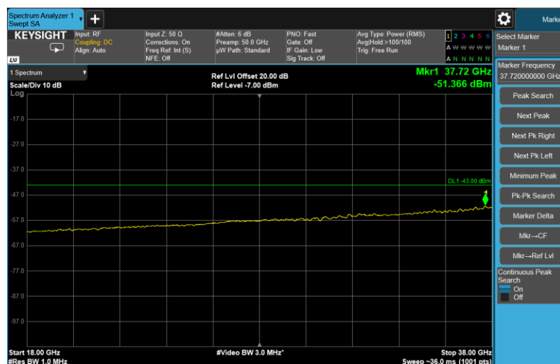
Channel: MIDDLE, Modulation: 16QAM, BW=20MHz, Range: 18GHz - 38GHz
