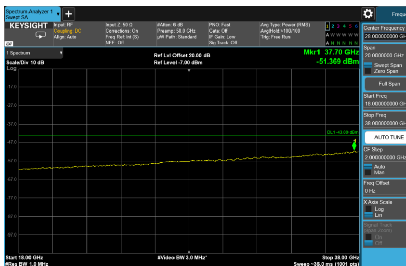
Channel: TOP, Modulation: 256QAM, BW=5MHz, Range: 18GHz - 38GHz
