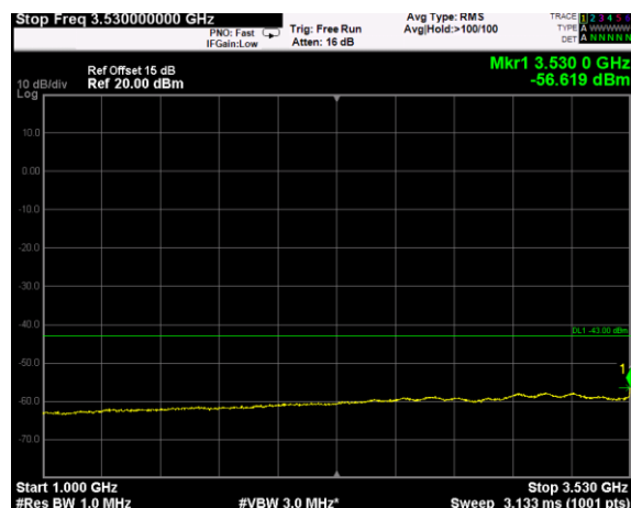
Channel: BOTTOM, Modulation: 256QAM, BW=15MHz, Range: 1GHz - 3530MHz
