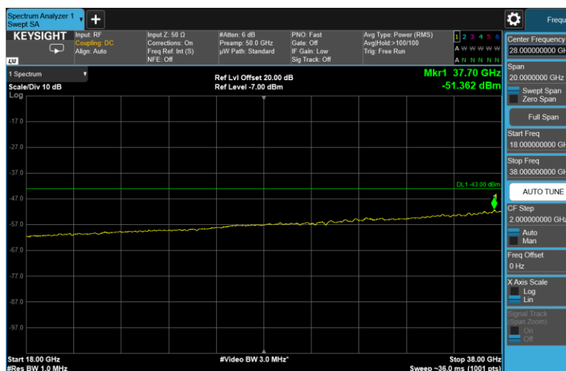
Channel: BOTTOM, Modulation: 16QAM, BW=10 MHz, Range: 18GHz - 38GHz
