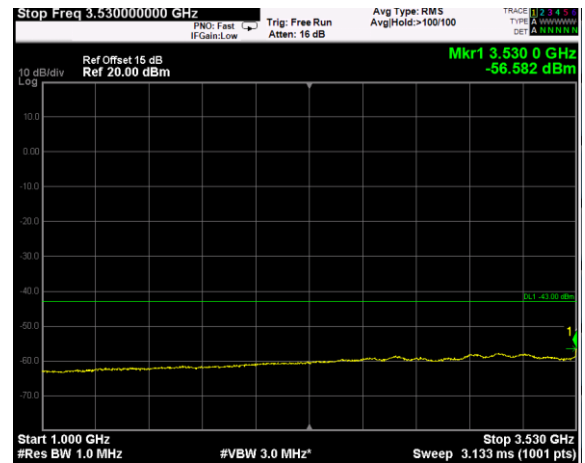
Channel: MIDDLE, Modulation: 16QAM, BW=20MHz, Range: 1GHz - 3530MHz
