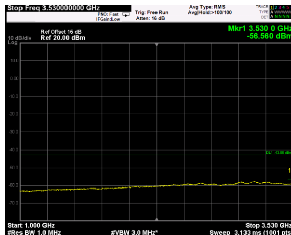
Channel: TOP, Modulation: 256QAM, BW=5MHz, Range: 1GHz - 3530MHz
