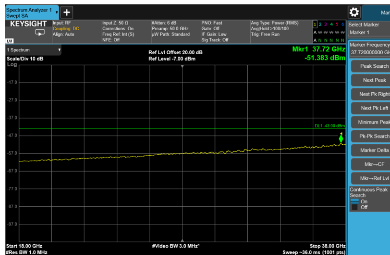
Channel: BOTTOM, Modulation: QPSK, BW=15MHz, Range: 18GHz - 38GHz
