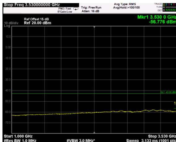
Channel: TOP, Modulation: QPSK, BW=15MHz, Range: 1GHz - 3530MHz
