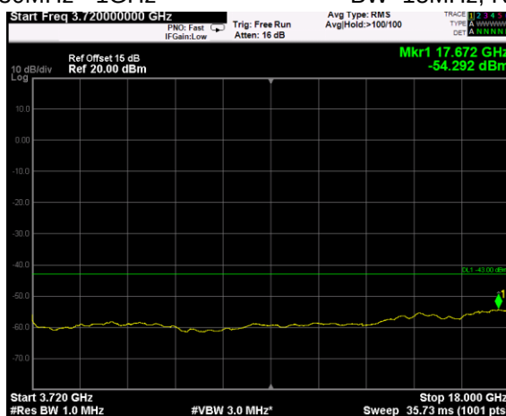
Channel: TOP, Modulation: 64QAM, BW=15MHz, Range: 3720MHz - 18GHz
