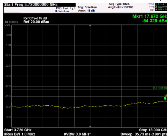
Channel: MIDDLE, Modulation: 16QAM, BW=10 MHz, Range: 3720MHz - 18GHz
