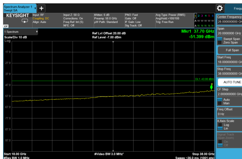
Channel: MIDDLE, Modulation: 64QAM, BW=20MHz, Range: 18GHz - 38GHz
