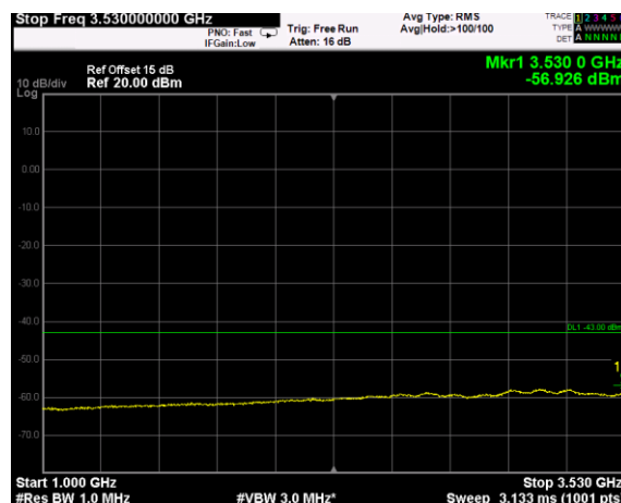
Channel: BOTTOM, Modulation: QPSK, BW=20MHz, Range: 1GHz - 3530MHz
