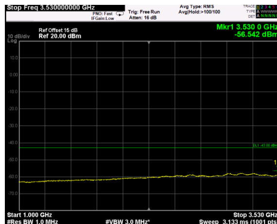
Channel: MIDDLE, Modulation: 16QAM, BW=5 MHz, Range: 1GHz - 3530MHz
