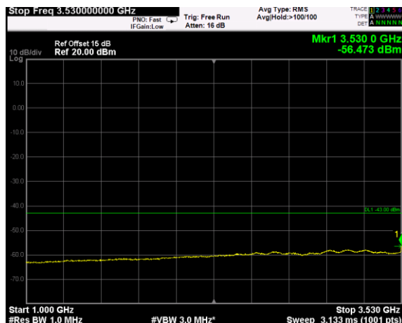
Channel: MIDDLE, Modulation: QPSK, BW=20MHz, Range: 1GHz - 3530MHz
