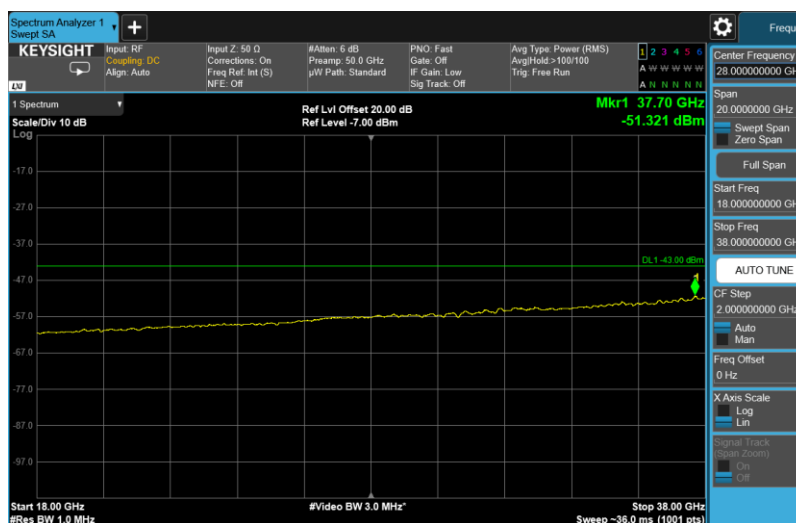
Channel: TOP, Modulation: 64QAM, BW=15MHz, Range: 18GHz - 38GHz
