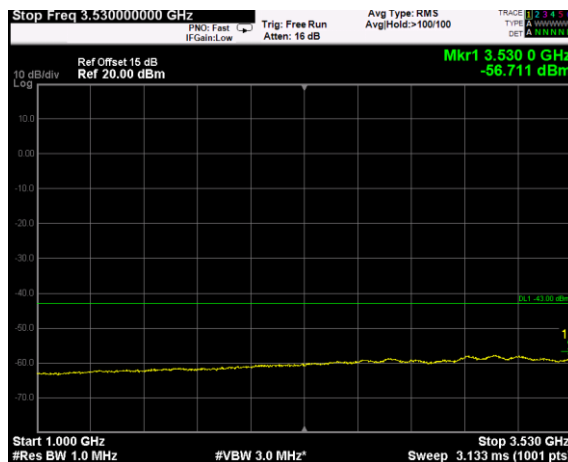
Channel: TOP, Modulation: 64QAM, BW=15MHz, Range: 1GHz - 3530MHz
