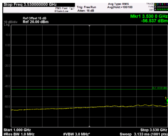
Channel: MIDDLE, Modulation: QPSK, BW=5 MHz, Range: 1GHz - 3530MHz
