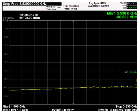
Channel: BOTTOM, Modulation: 64QAM, BW=5 MHz, Range: 1GHz - 3530MHz
