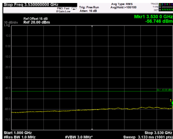
Channel: MIDDLE, Modulation: 16QAM, BW=15MHz, Range: 1GHz - 3530MHz
