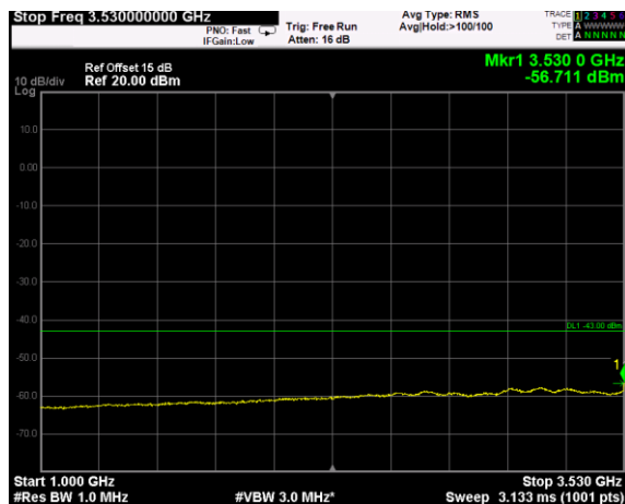
Channel: BOTTOM, Modulation: 64QAM, BW=15MHz, Range: 1GHz - 3530MHz
