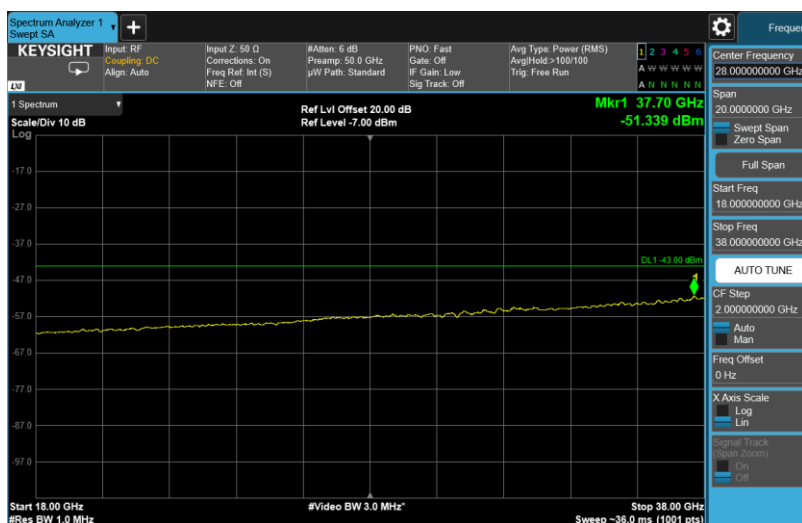
Channel: MIDDLE, Modulation: QPSK, BW=20MHz, Range: 18GHz - 38GHz
