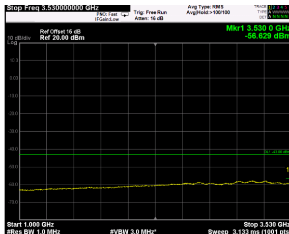
Channel: MIDDLE, Modulation: 256QAM, BW=5MHz, Range: 1GHz - 3530MHz
