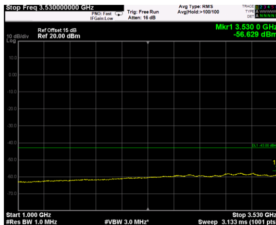
Channel: MIDDLE, Modulation: 256QAM, BW=15MHz, Range: 1GHz - 3530MHz
