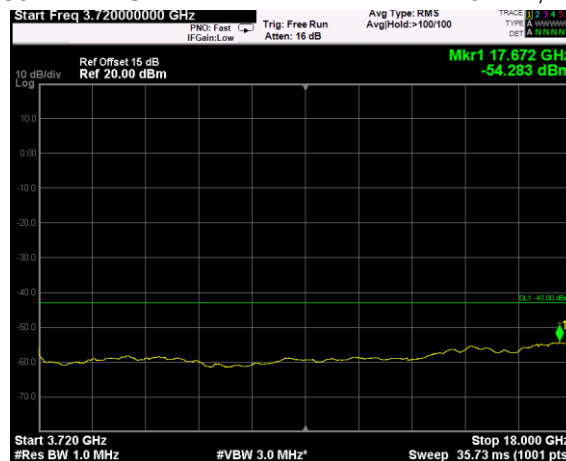
Channel: BOTTOM, Modulation: 16QAM, BW=20MHz, Range: 3720MHz - 18GHz
