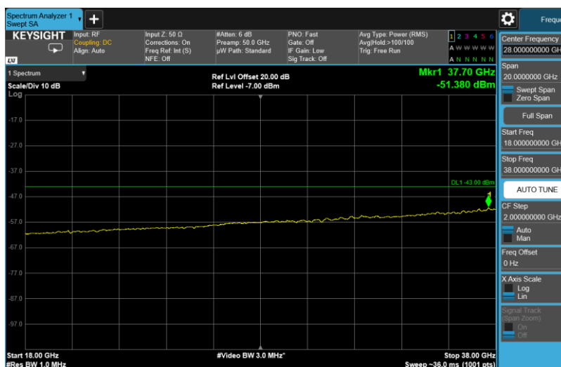
Channel: TOP, Modulation: QPSK, BW=5MHz, Range: 18GHz - 38GHz
