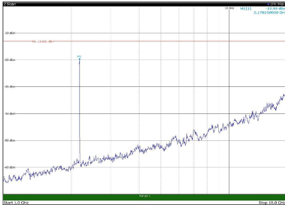
Channel: TOP, Modulation: 16QAM, BW=15MHz, Range: 1GHz - 18GHz, Polarization: Horizontal
