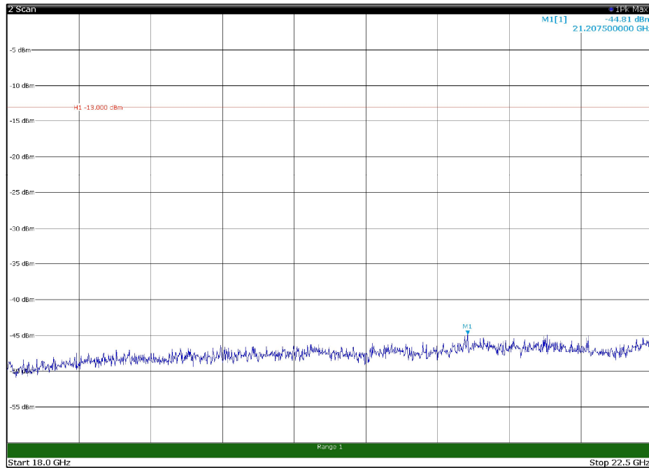
Channel: TOP, Modulation: 16QAM, BW=15MHz, Range: 18GHz - 22.5GHz, Polarization: Horizontal
