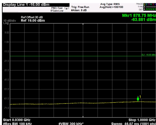
Channel: BOTTOM, Modulation: QPSK, BW=20MHz, Range: Lower
