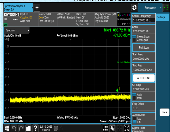
3DH5-Ant1-2480-30~1000-PASS
