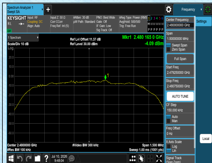
3DH5-Ant1-2480-0~Reference-PASS
