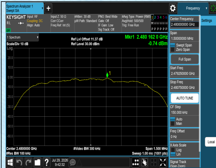
3DH5-Ant1-2480-0~Reference-PASS
