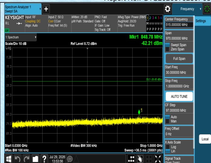
11N20SISO-Ant1-2412-30~1000-PASS
