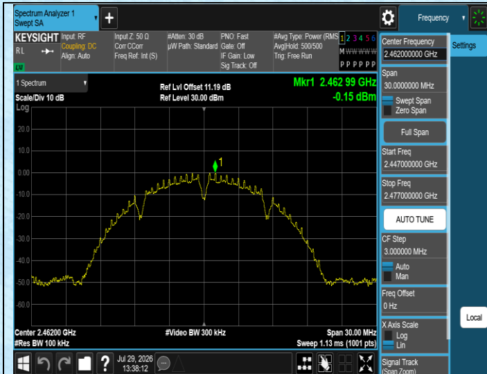
11B-Ant1-2462-0~Reference-PASS
