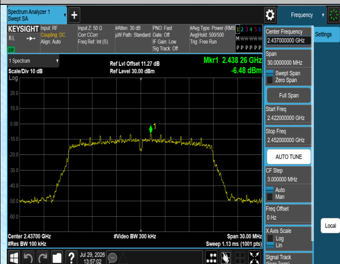
11N20SISO-Ant1-2437-0~Reference-PASS
