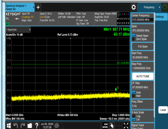
11N20SISO-Ant1-2437-30~1000-PASS
