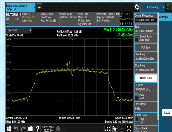
11N20SISO-Ant1-2412-0~Reference-PASS
