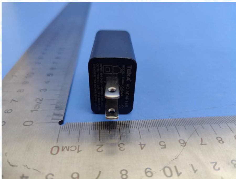
Photo 7 Adapter Appearance
