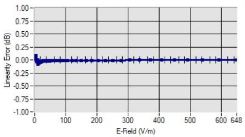
Linearity
