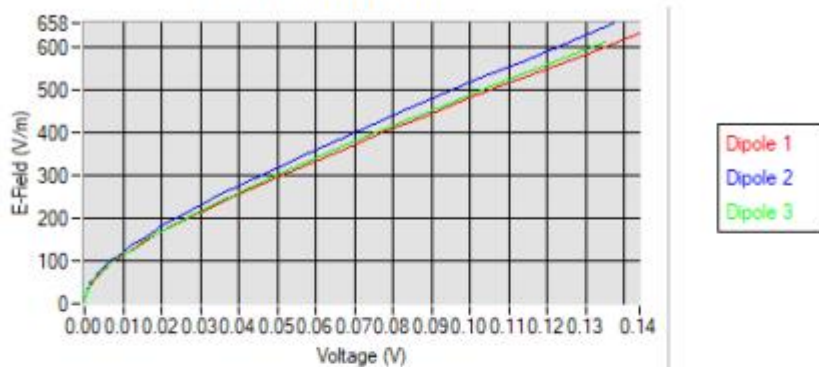
Calibration curves
