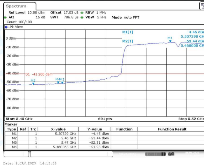
11N40SISO_Ant1_Low_5510_Peak
