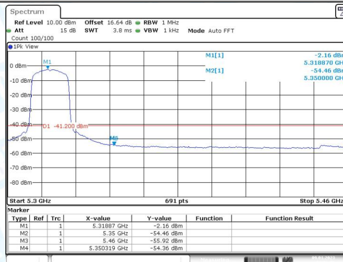
11A_Ant1_High_5320_AV
