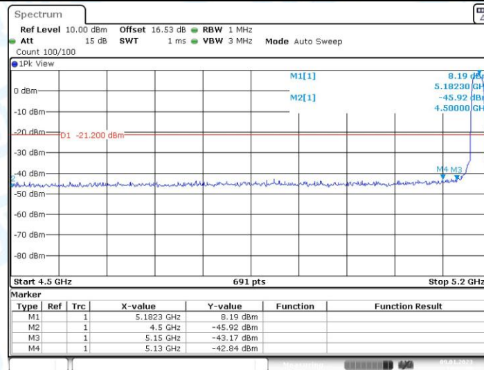
11A_Ant1_Low_5180_Peak
