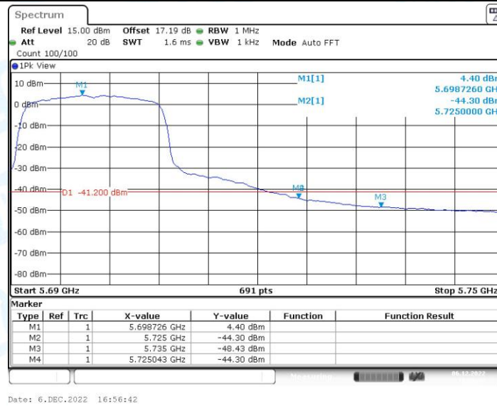
11A_Ant1_High_5700_Peak
