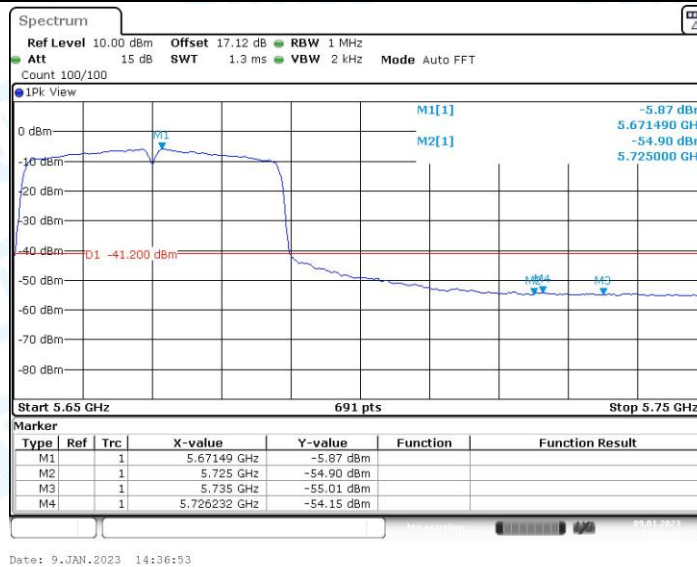
11AC40SISO_Ant1_High_5670_Peak
