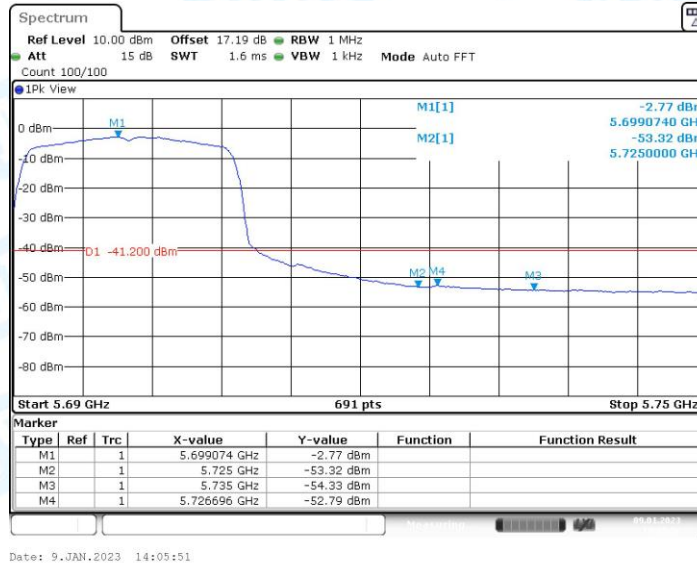
11N20SISO_Ant1_High_5700_Peak
