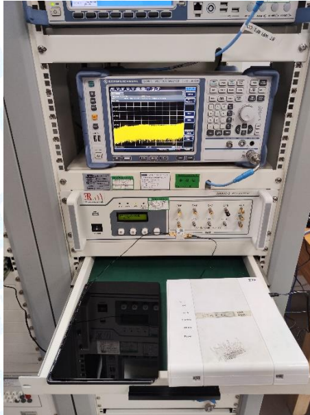
Photo of Setup for DFS Test
