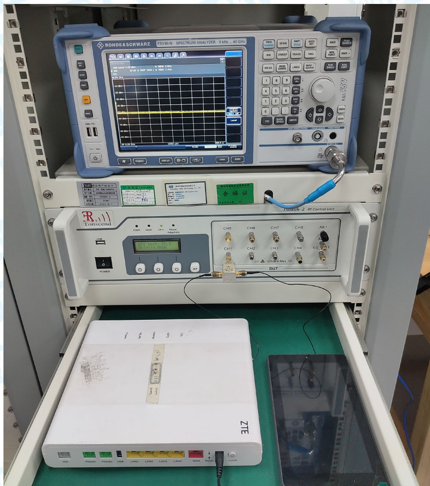
Photo of Setup for DFS Test
