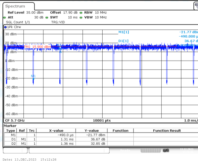
11AC20SISO_Ant1_5720
