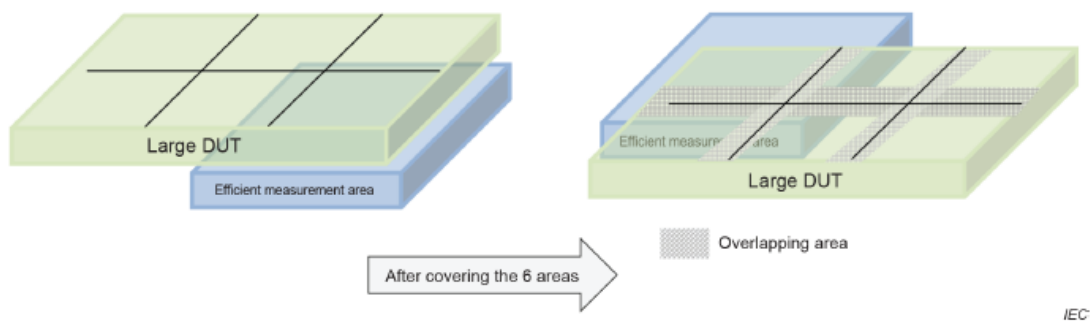
Figure 5 – Measurements performed by shifting a large device over the efficient measurement area of the system including overlapping areas – in this case: six tests performed
